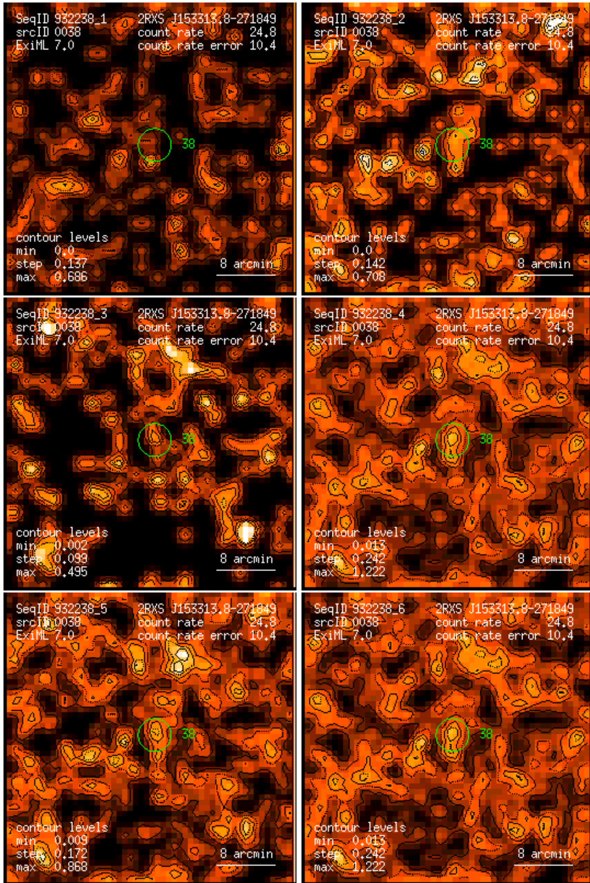
Figure 38: RASS 932238: detection 0038: band rate images, Gaussian filter: (1) PSPC channels 11 – 41, (2) 52 – 90, (3) 91 – 201, (4) 11 – 235, (5) 52 – 201, (6) 11 – 201. Broad band rates in counts/ks. Band rate contour levels in counts/ks/arcmin 2 .
