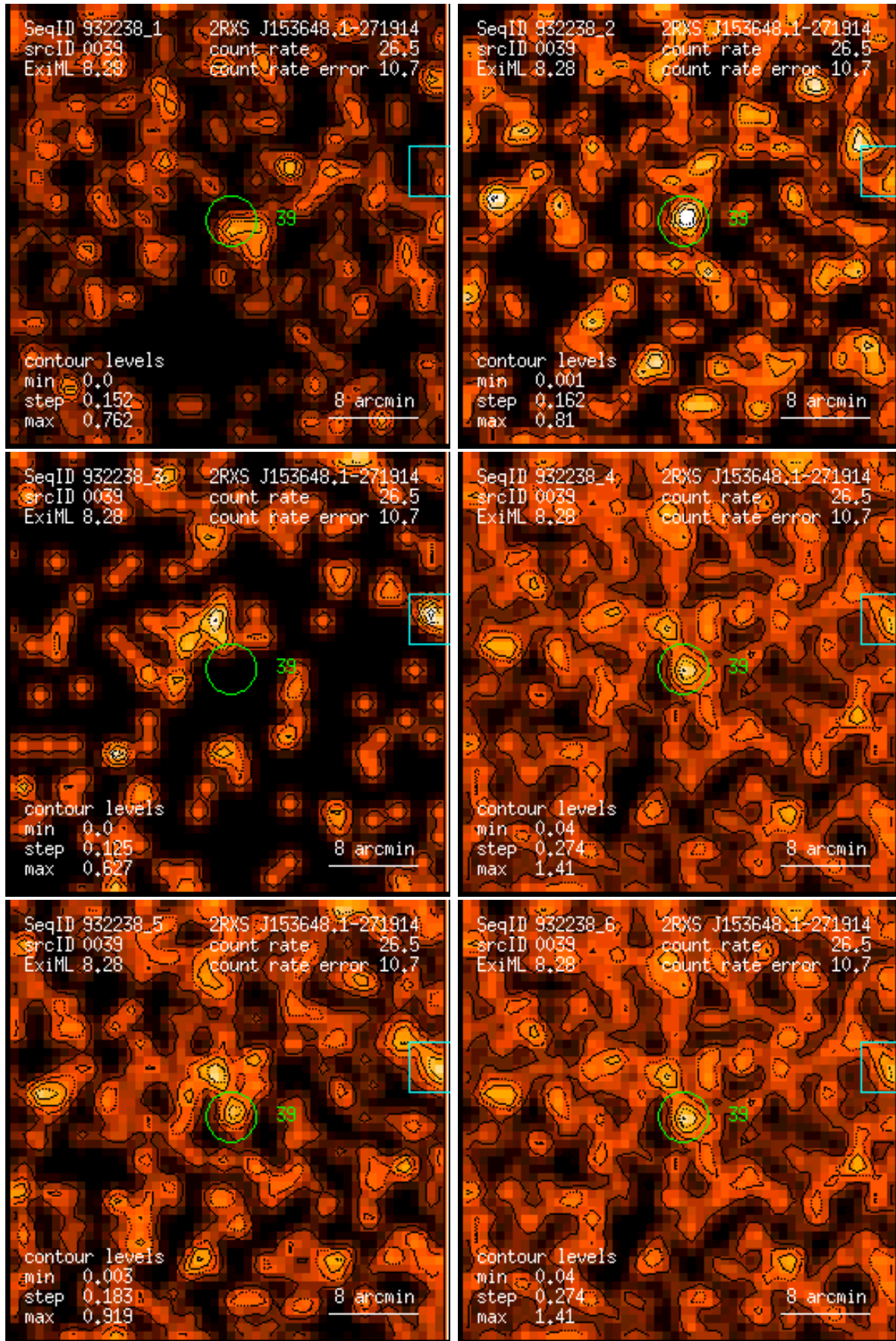
Figure 39: RASS 932238: detection 0039: band rate images, Gaussian filter: (1) PSPC channels 11 – 41, (2) 52 – 90, (3) 91 – 201, (4) 11 – 235, (5) 52 – 201, (6) 11 – 201. Broad band rates in counts/ks. Band rate contour levels in counts/ks/arcmin 2 .
