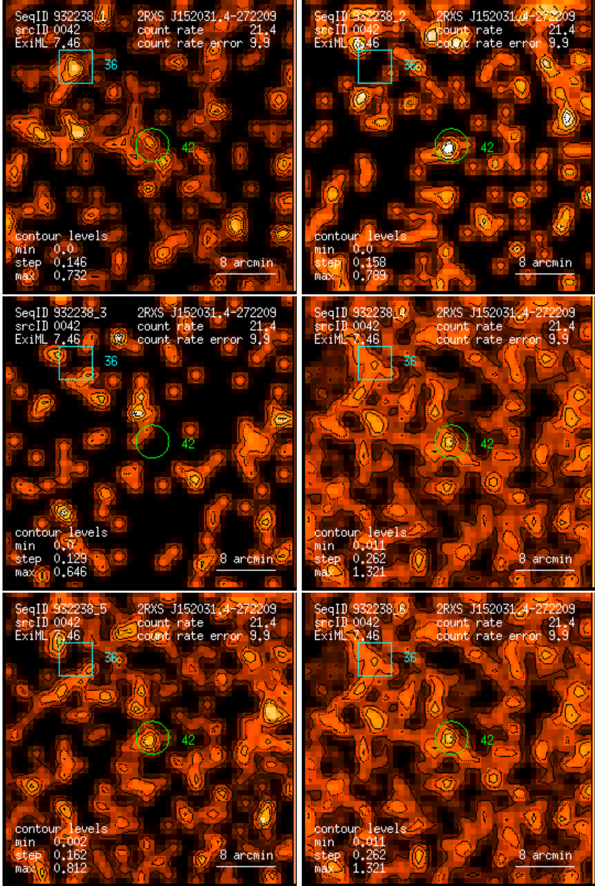
Figure 42: RASS 932238: detection 0042: band rate images, Gaussian filter: (1) PSPC channels 11 – 41, (2) 52 – 90, (3) 91 – 201, (4) 11 – 235, (5) 52 – 201, (6) 11 – 201. Broad band rates in counts/ks. Band rate contour levels in counts/ks/arcmin 2 .
