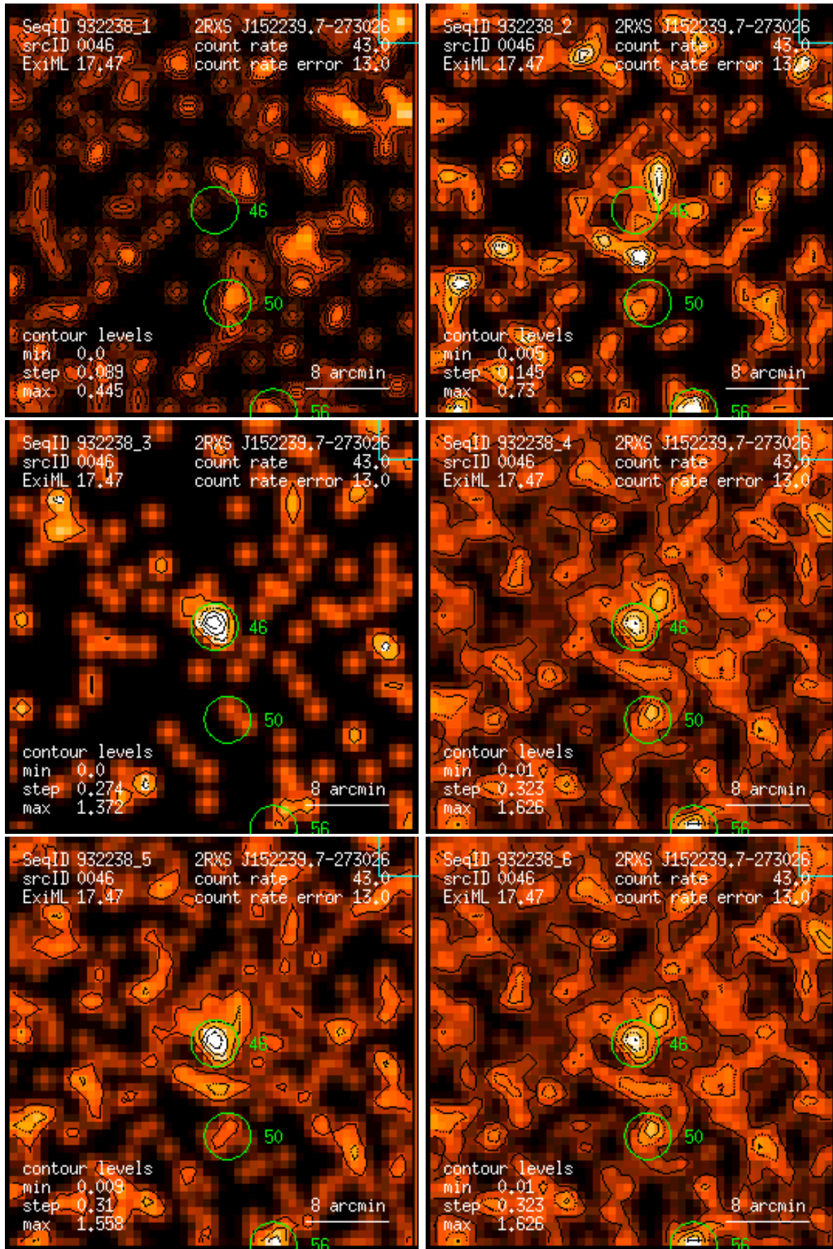
Figure 46: RASS 932238: detection 0046: band rate images, Gaussian filter: (1) PSPC channels 11 – 41, (2) 52 – 90, (3) 91 – 201, (4) 11 – 235, (5) 52 – 201, (6) 11 – 201. Broad band rates in counts/ks. Band rate contour levels in counts/ks/arcmin 2 .
