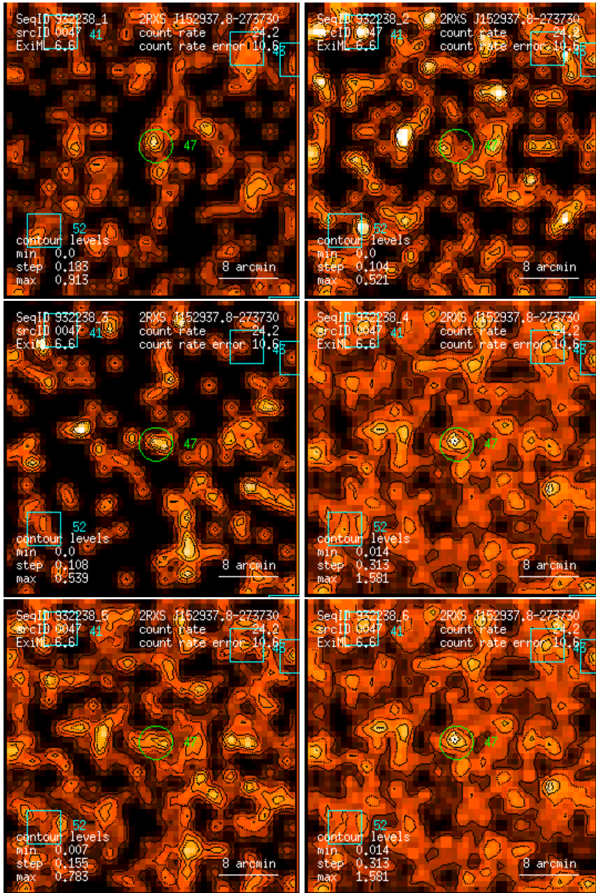
Figure 47: RASS 932238: detection 0047: band rate images, Gaussian filter: (1) PSPC channels 11 – 41, (2) 52 – 90, (3) 91 – 201, (4) 11 – 235, (5) 52 – 201, (6) 11 – 201. Broad band rates in counts/ks. Band rate contour levels in counts/ks/arcmin 2 .
