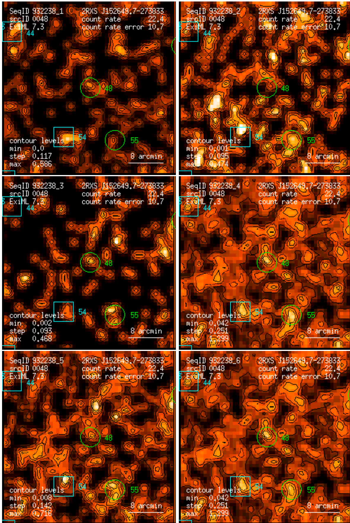
Figure 48: RASS 932238: detection 0048: band rate images, Gaussian filter: (1) PSPC channels 11 – 41, (2) 52 – 90, (3) 91 – 201, (4) 11 – 235, (5) 52 – 201, (6) 11 – 201. Broad band rates in counts/ks. Band rate contour levels in counts/ks/arcmin 2 .
