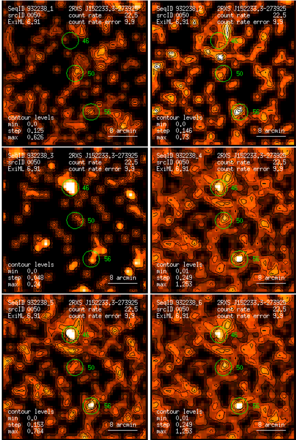
Figure 50: RASS 932238: detection 0050: band rate images, Gaussian filter: (1) PSPC channels 11 – 41, (2) 52 – 90, (3) 91 – 201, (4) 11 – 235, (5) 52 – 201, (6) 11 – 201. Broad band rates in counts/ks. Band rate contour levels in counts/ks/arcmin 2 .
