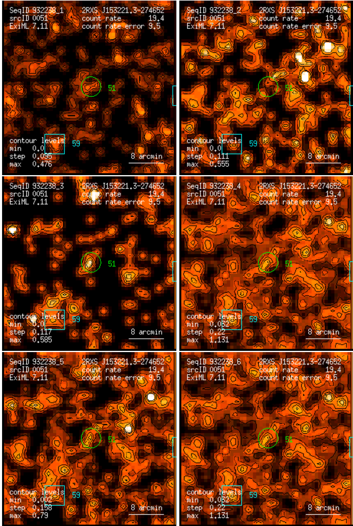
Figure 51: RASS 932238: detection 0051: band rate images, Gaussian filter: (1) PSPC channels 11 – 41, (2) 52 – 90, (3) 91 – 201, (4) 11 – 235, (5) 52 – 201, (6) 11 – 201. Broad band rates in counts/ks. Band rate contour levels in counts/ks/arcmin 2 .
