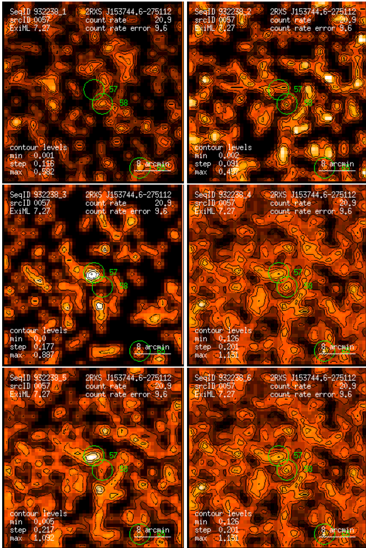
Figure 57: RASS 932238: detection 0057: band rate images, Gaussian filter: (1) PSPC channels 11 – 41, (2) 52 – 90, (3) 91 – 201, (4) 11 – 235, (5) 52 – 201, (6) 11 – 201. Broad band rates in counts/ks. Band rate contour levels in counts/ks/arcmin 2 .
