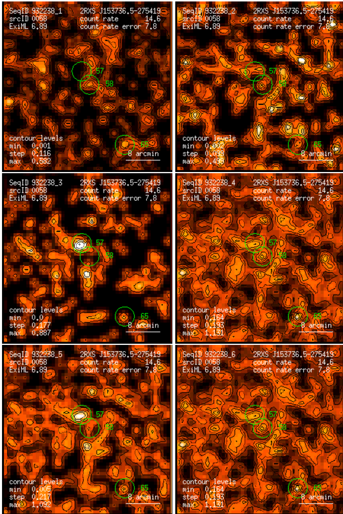
Figure 58: RASS 932238: detection 0058: band rate images, Gaussian filter: (1) PSPC channels 11 – 41, (2) 52 – 90, (3) 91 – 201, (4) 11 – 235, (5) 52 – 201, (6) 11 – 201. Broad band rates in counts/ks. Band rate contour levels in counts/ks/arcmin 2 .
