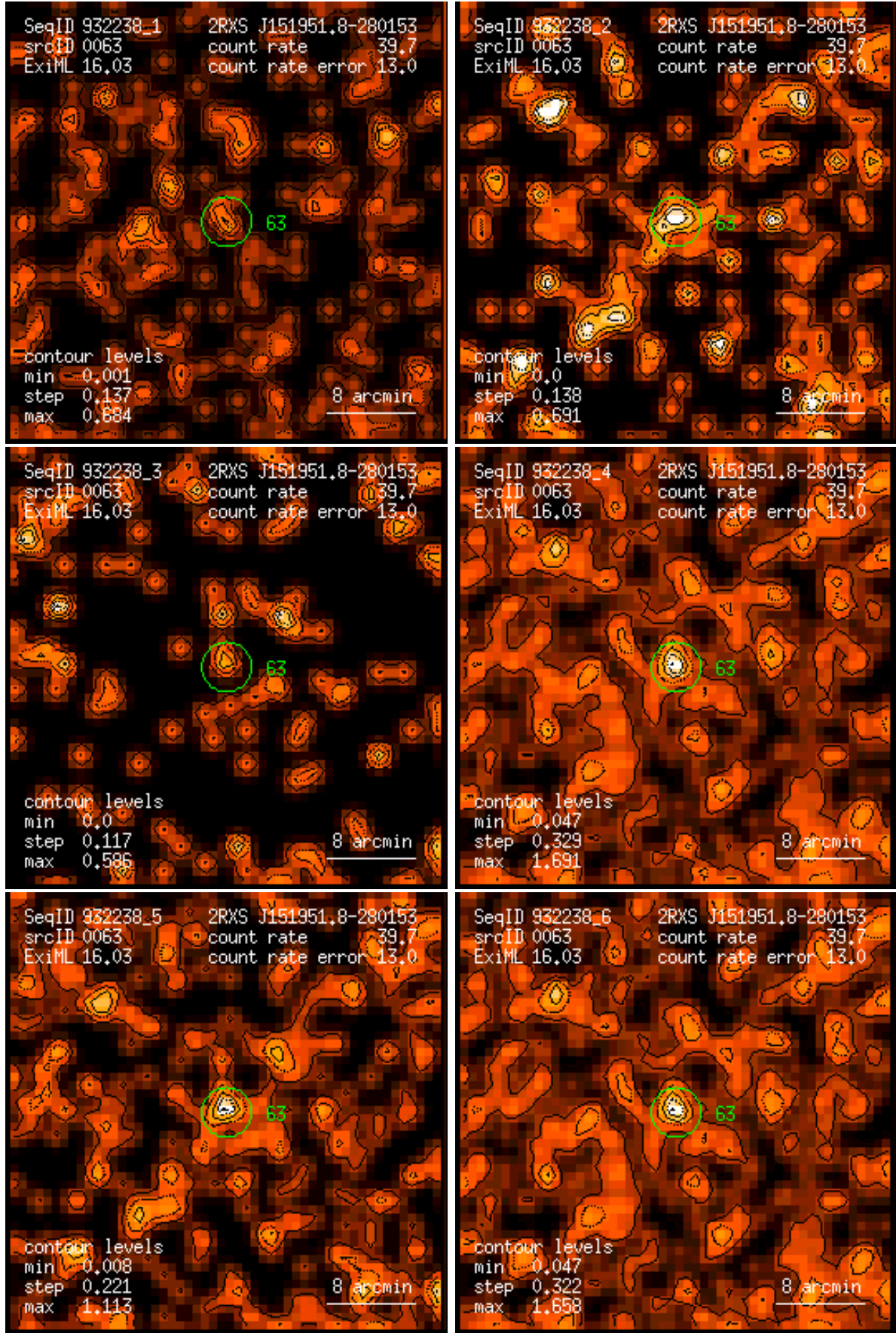
Figure 63: RASS 932238: detection 0063: band rate images, Gaussian filter: (1) PSPC channels 11 – 41, (2) 52 – 90, (3) 91 – 201, (4) 11 – 235, (5) 52 – 201, (6) 11 – 201. Broad band rates in counts/ks. Band rate contour levels in counts/ks/arcmin 2 .
