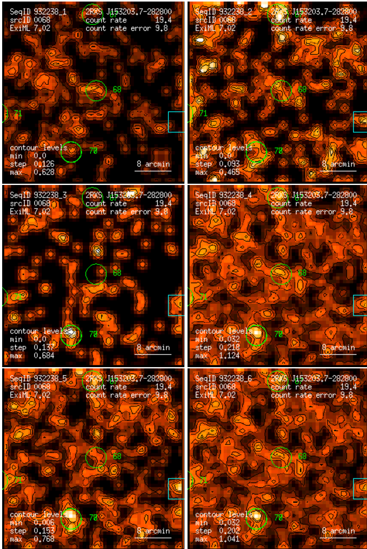
Figure 68: RASS 932238: detection 0068: band rate images, Gaussian filter: (1) PSPC channels 11 – 41, (2) 52 – 90, (3) 91 – 201, (4) 11 – 235, (5) 52 – 201, (6) 11 – 201. Broad band rates in counts/ks. Band rate contour levels in counts/ks/arcmin 2 .
