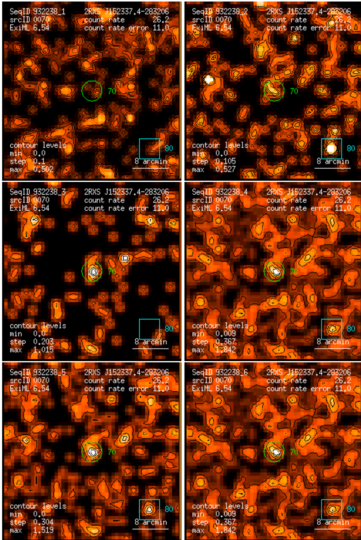
Figure 70: RASS 932238: detection 0070: band rate images, Gaussian filter: (1) PSPC channels 11 – 41, (2) 52 – 90, (3) 91 – 201, (4) 11 – 235, (5) 52 – 201, (6) 11 – 201. Broad band rates in counts/ks. Band rate contour levels in counts/ks/arcmin 2 .
