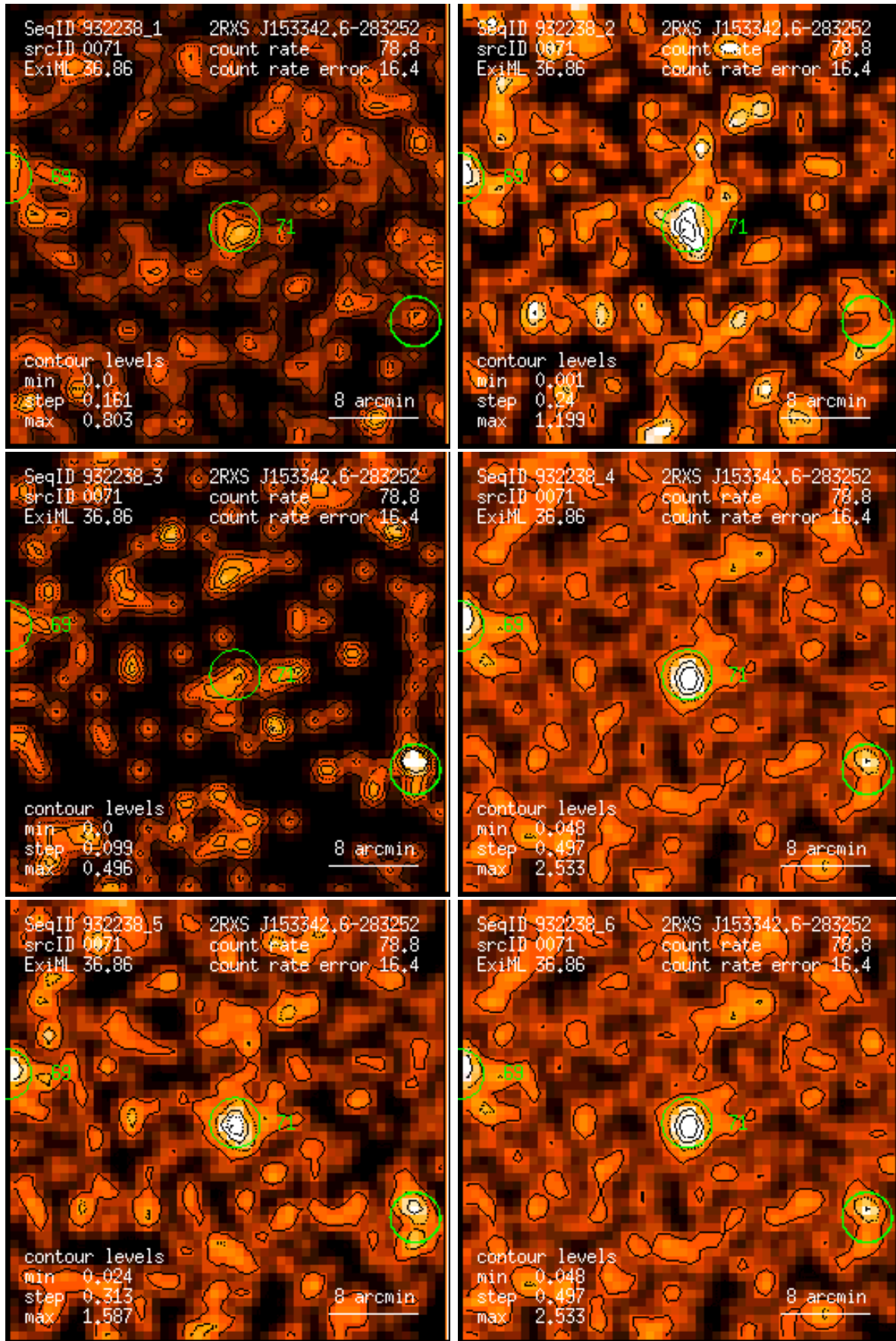
Figure 71: RASS 932238: detection 0071: band rate images, Gaussian filter: (1) PSPC channels 11 – 41, (2) 52 – 90, (3) 91 – 201, (4) 11 – 235, (5) 52 – 201, (6) 11 – 201. Broad band rates in counts/ks. Band rate contour levels in counts/ks/arcmin 2 .
