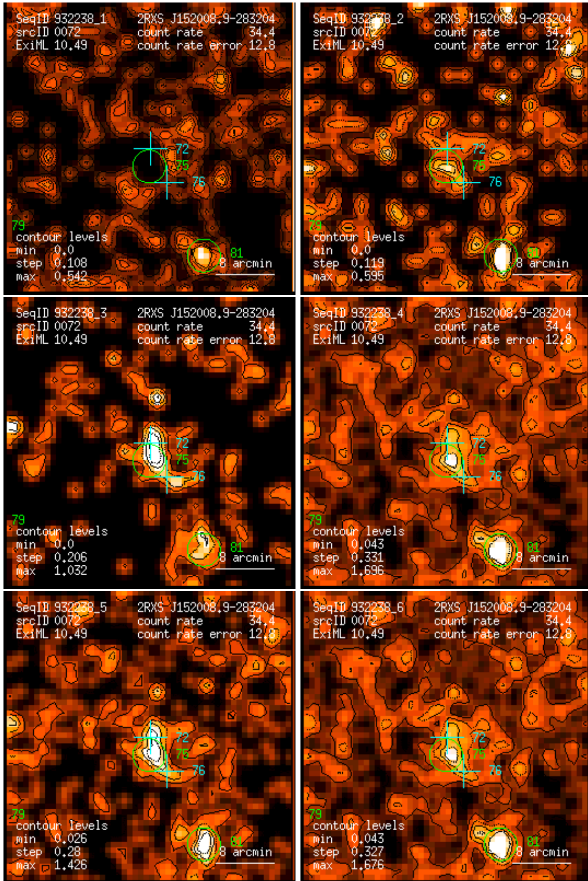
Figure 72: RASS 932238: detection 0072: band rate images, Gaussian filter: (1) PSPC channels 11 – 41, (2) 52 – 90, (3) 91 – 201, (4) 11 – 235, (5) 52 – 201, (6) 11 – 201. Broad band rates in counts/ks. Band rate contour levels in counts/ks/arcmin 2 .
