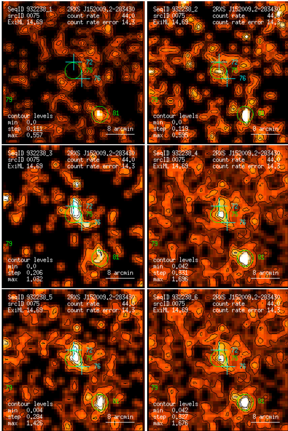
Figure 75: RASS 932238: detection 0075: band rate images, Gaussian filter: (1) PSPC channels 11 – 41, (2) 52 – 90, (3) 91 – 201, (4) 11 – 235, (5) 52 – 201, (6) 11 – 201. Broad band rates in counts/ks. Band rate contour levels in counts/ks/arcmin 2 .
