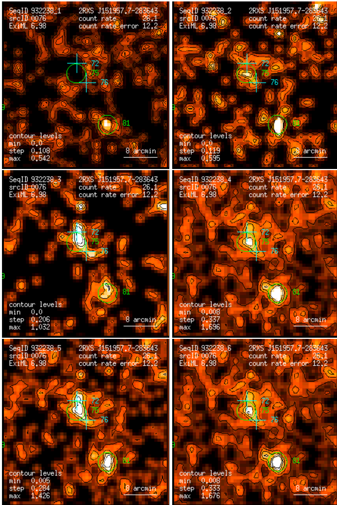
Figure 76: RASS 932238: detection 0076: band rate images, Gaussian filter: (1) PSPC channels 11 – 41, (2) 52 – 90, (3) 91 – 201, (4) 11 – 235, (5) 52 – 201, (6) 11 – 201. Broad band rates in counts/ks. Band rate contour levels in counts/ks/arcmin 2 .
