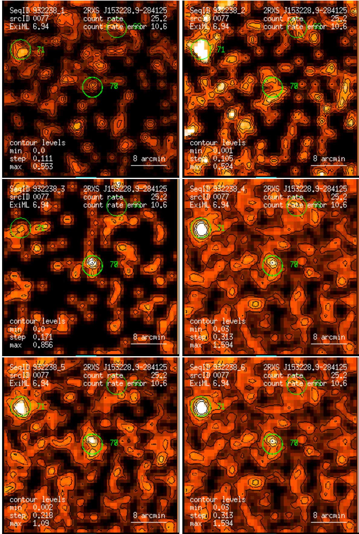
Figure 77: RASS 932238: detection 0077: band rate images, Gaussian filter: (1) PSPC channels 11 – 41, (2) 52 – 90, (3) 91 – 201, (4) 11 – 235, (5) 52 – 201, (6) 11 – 201. Broad band rates in counts/ks. Band rate contour levels in counts/ks/arcmin 2 .
