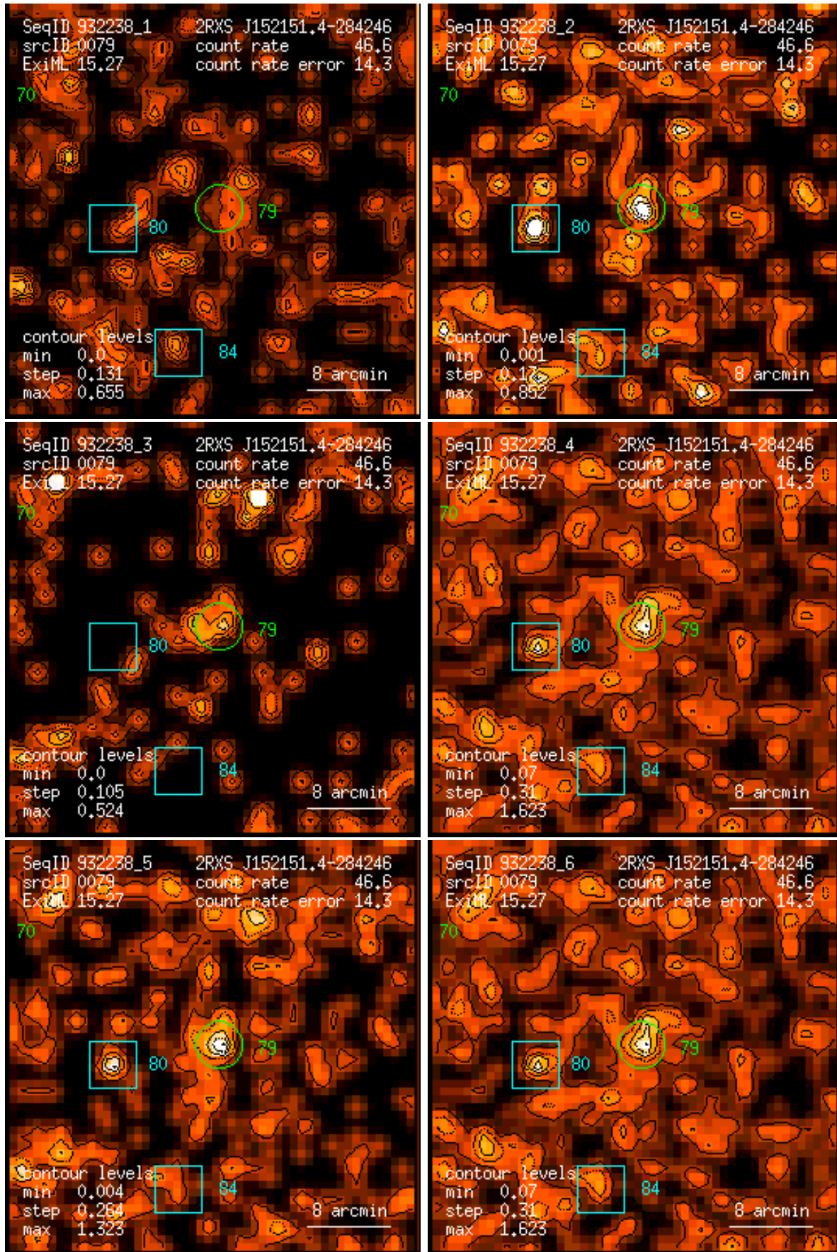
Figure 79: RASS 932238: detection 0079: band rate images, Gaussian filter: (1) PSPC channels 11 – 41, (2) 52 – 90, (3) 91 – 201, (4) 11 – 235, (5) 52 – 201, (6) 11 – 201. Broad band rates in counts/ks. Band rate contour levels in counts/ks/arcmin 2 .
