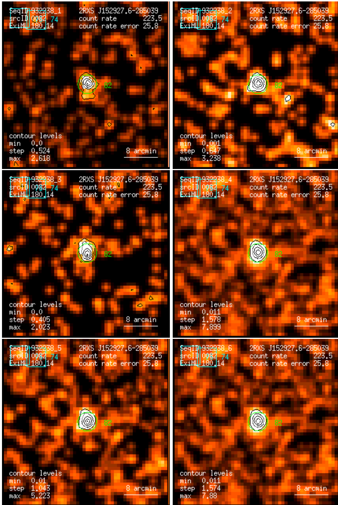
Figure 82: RASS 932238: detection 0082: band rate images, Gaussian filter: (1) PSPC channels 11 – 41, (2) 52 – 90, (3) 91 – 201, (4) 11 – 235, (5) 52 – 201, (6) 11 – 201. Broad band rates in counts/ks. Band rate contour levels in counts/ks/arcmin 2 .
