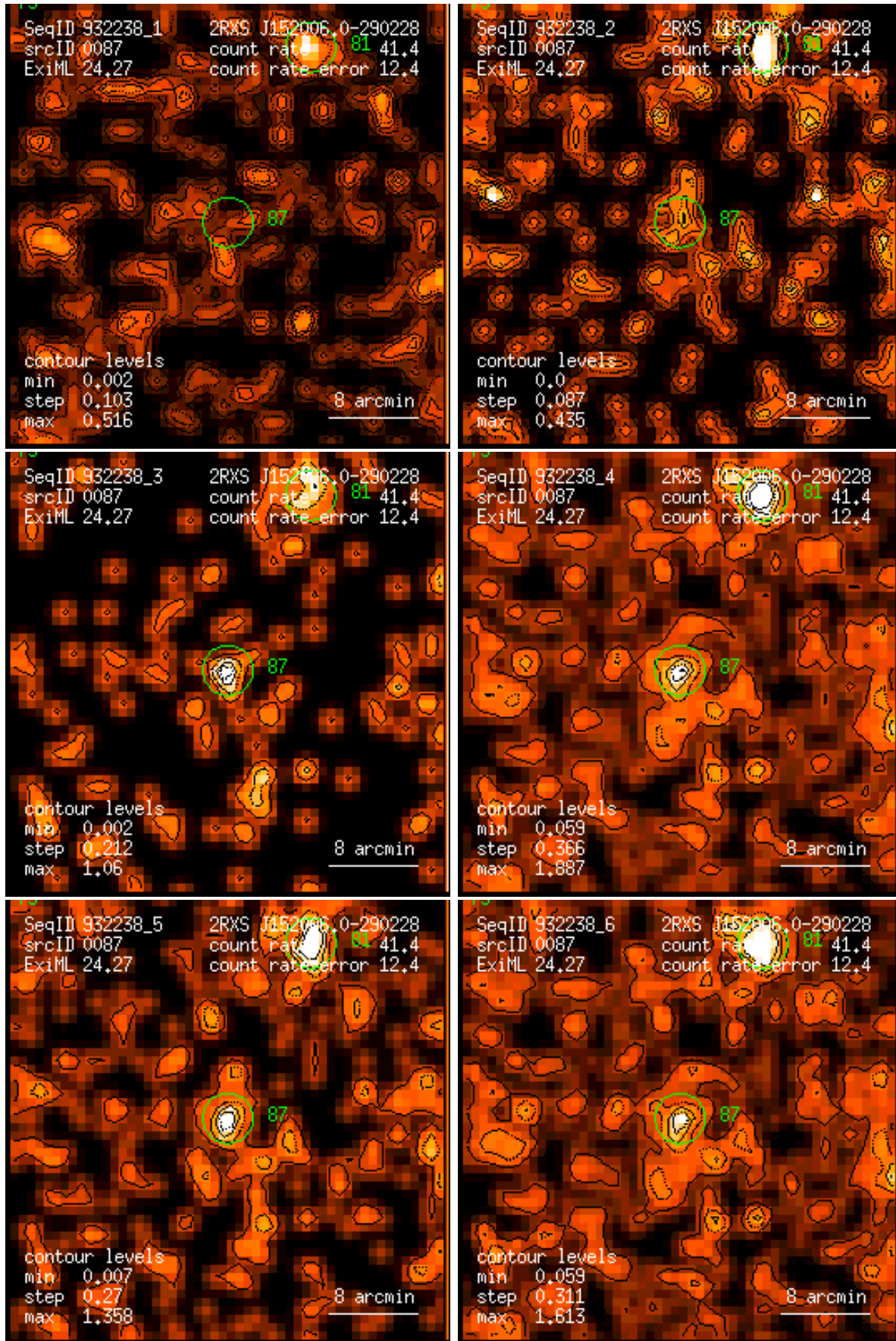
Figure 87: RASS 932238: detection 0087: band rate images, Gaussian filter: (1) PSPC channels 11 – 41, (2) 52 – 90, (3) 91 – 201, (4) 11 – 235, (5) 52 – 201, (6) 11 – 201. Broad band rates in counts/ks. Band rate contour levels in counts/ks/arcmin 2 .
