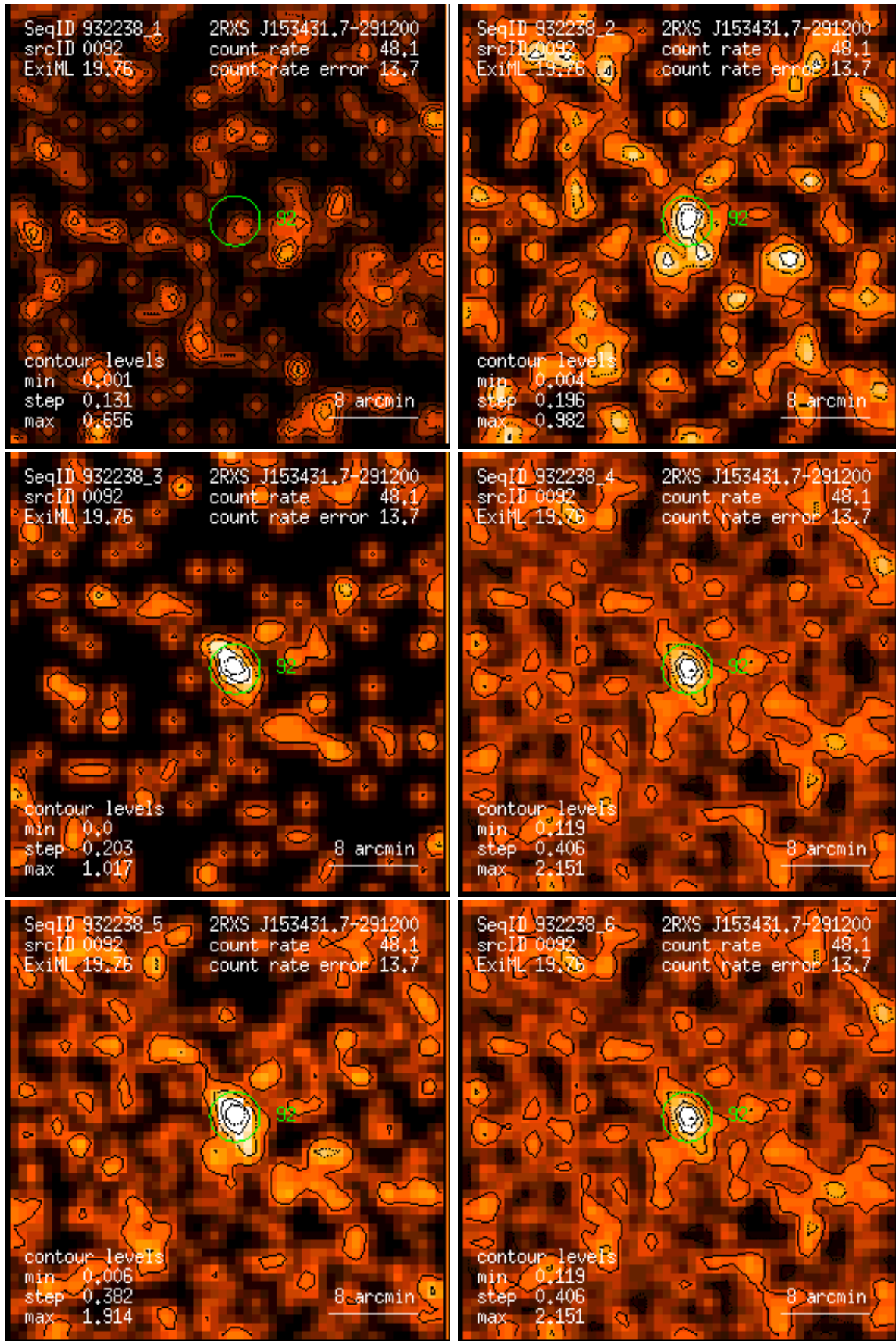
Figure 92: RASS 932238: detection 0092: band rate images, Gaussian filter: (1) PSPC channels 11 – 41, (2) 52 – 90, (3) 91 – 201, (4) 11 – 235, (5) 52 – 201, (6) 11 – 201. Broad band rates in counts/ks. Band rate contour levels in counts/ks/arcmin 2 .
