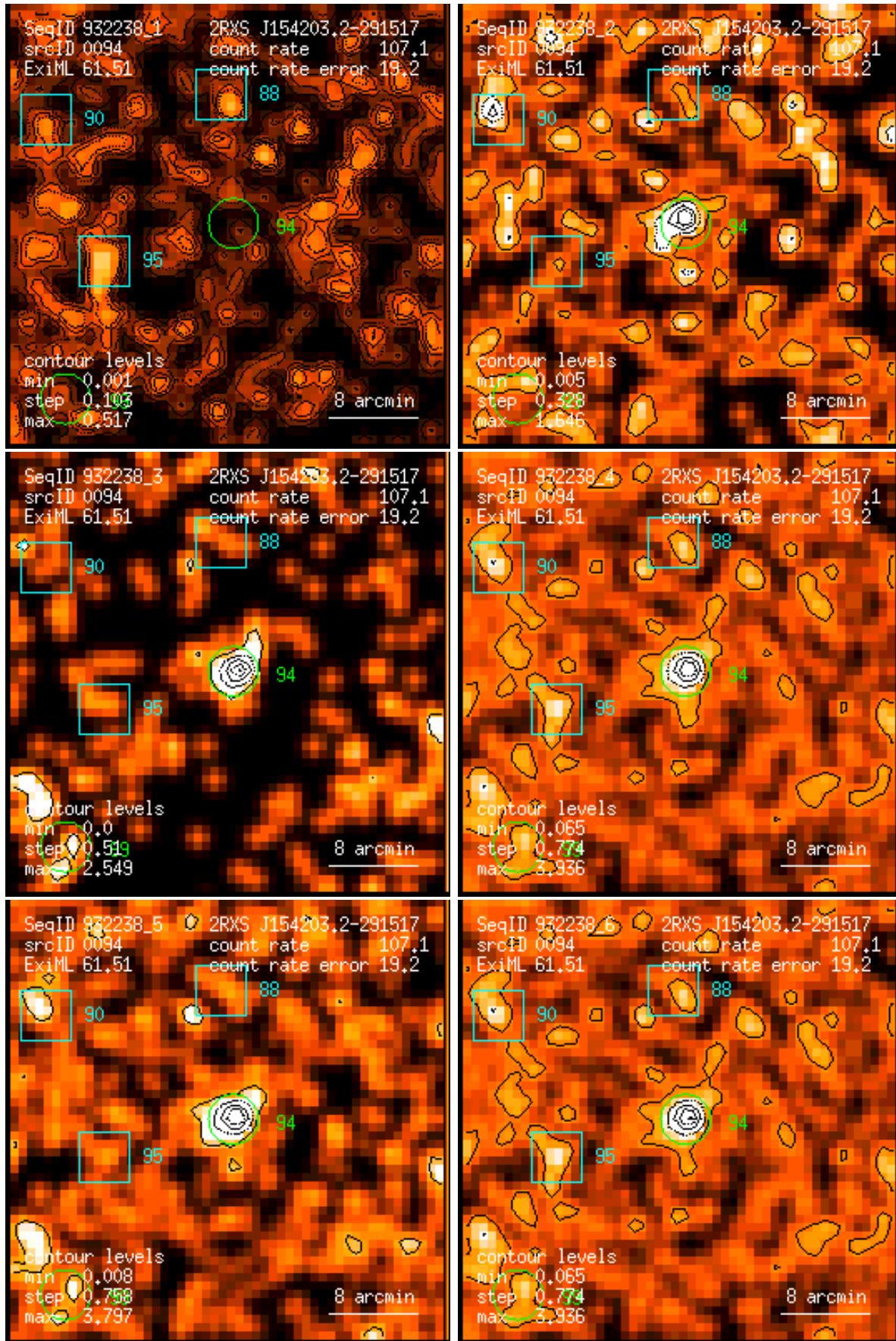
Figure 94: RASS 932238: detection 0094: band rate images, Gaussian filter: (1) PSPC channels 11 – 41, (2) 52 – 90, (3) 91 – 201, (4) 11 – 235, (5) 52 – 201, (6) 11 – 201. Broad band rates in counts/ks. Band rate contour levels in counts/ks/arcmin 2 .
