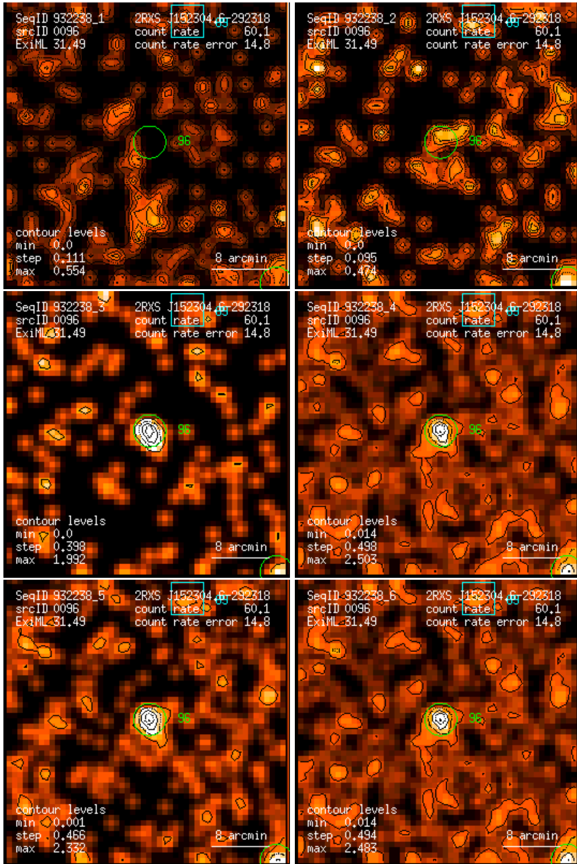
Figure 96: RASS 932238: detection 0096: band rate images, Gaussian filter: (1) PSPC channels 11 – 41, (2) 52 – 90, (3) 91 – 201, (4) 11 – 235, (5) 52 – 201, (6) 11 – 201. Broad band rates in counts/ks. Band rate contour levels in counts/ks/arcmin 2 .
