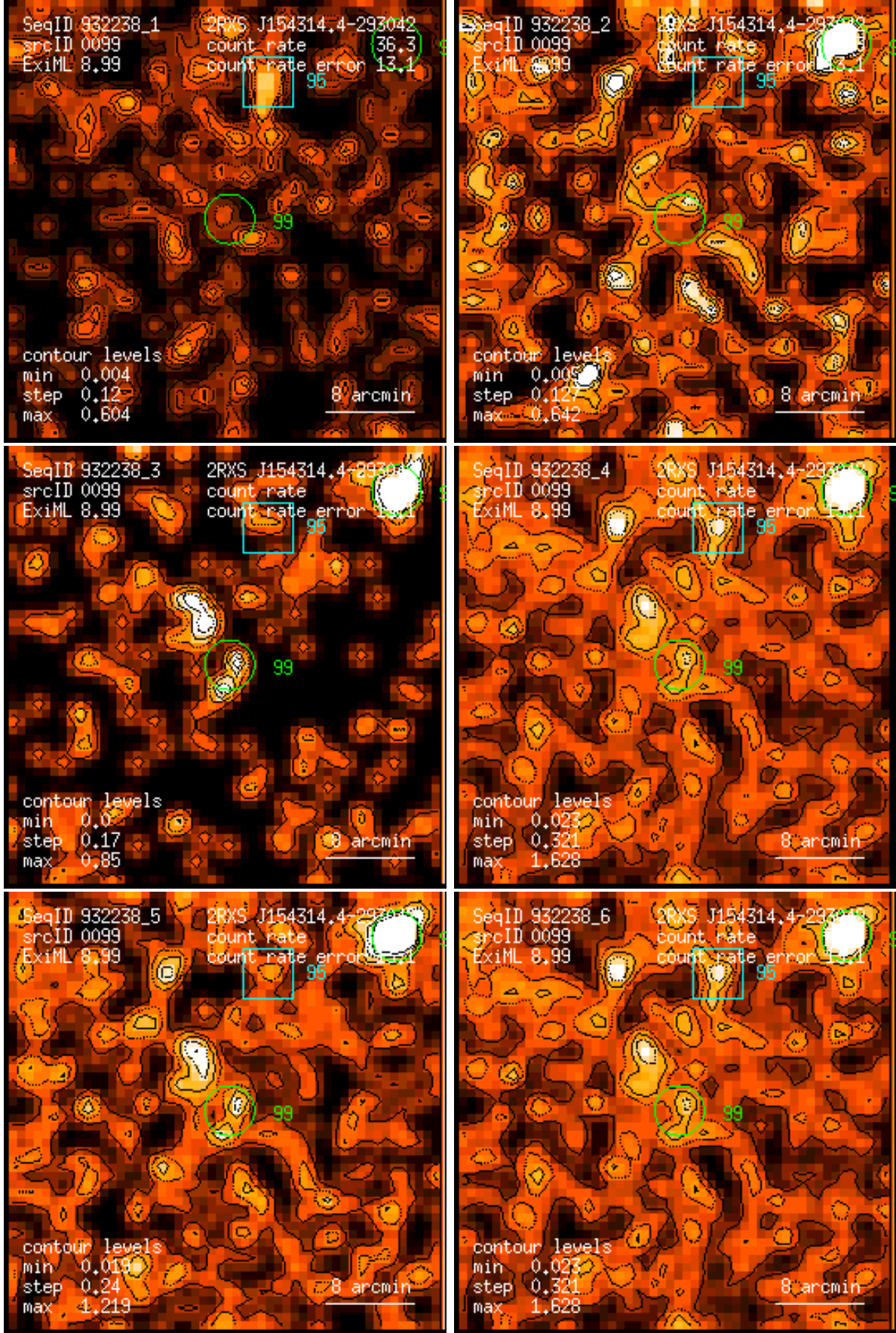
Figure 99: RASS 932238: detection 0099: band rate images, Gaussian filter: (1) PSPC channels 11 – 41, (2) 52 – 90, (3) 91 – 201, (4) 11 – 235, (5) 52 – 201, (6) 11 – 201. Broad band rates in counts/ks. Band rate contour levels in counts/ks/arcmin 2 .
