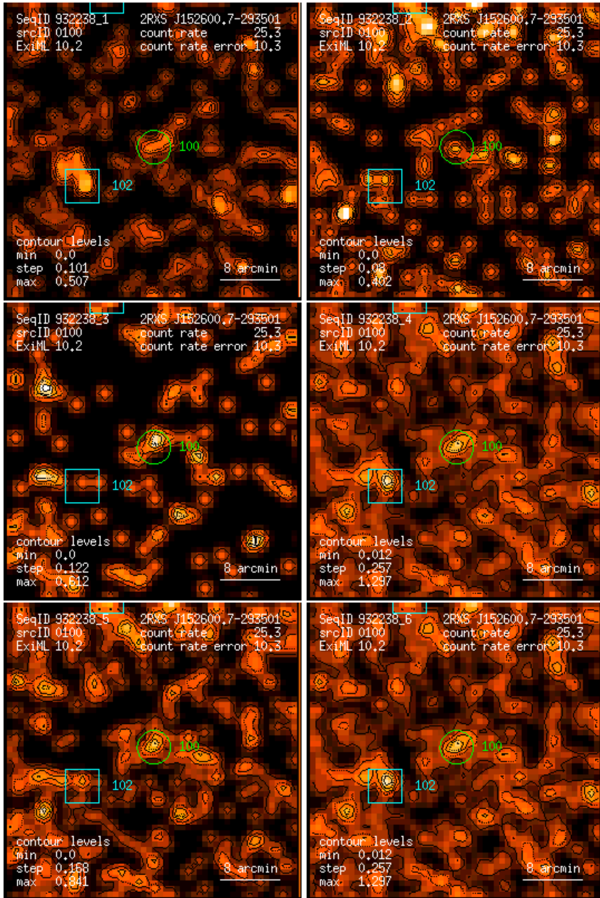
Figure 100: RASS 932238: detection 0100: band rate images, Gaussian filter: (1) PSPC channels 11 – 41, (2) 52 – 90, (3) 91 – 201, (4) 11 – 235, (5) 52 – 201, (6) 11 – 201. Broad band rates in counts/ks. Band rate contour levels in counts/ks/arcmin 2 .
