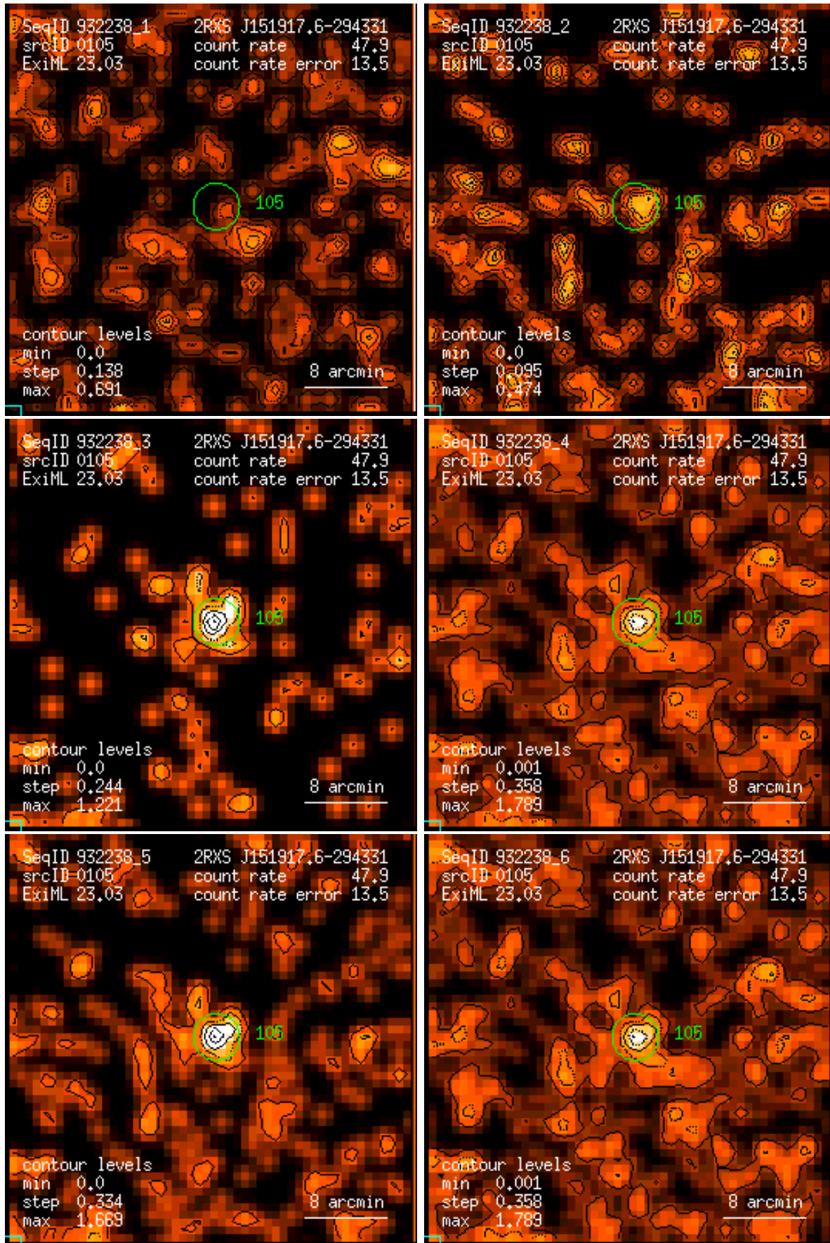
Figure 105: RASS 932238: detection 0105: band rate images, Gaussian filter: (1) PSPC channels 11 – 41, (2) 52 – 90, (3) 91 – 201, (4) 11 – 235, (5) 52 – 201, (6) 11 – 201. Broad band rates in counts/ks. Band rate contour levels in counts/ks/arcmin 2 .
