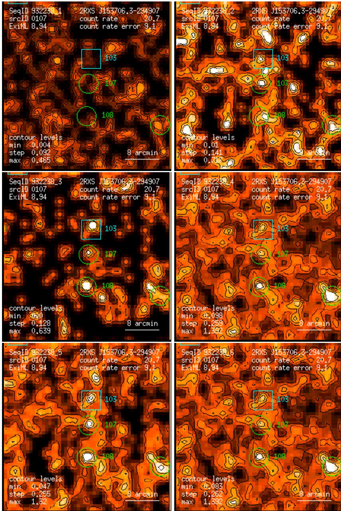
Figure 107: RASS 932238: detection 0107: band rate images, Gaussian filter: (1) PSPC channels 11 – 41, (2) 52 – 90, (3) 91 – 201, (4) 11 – 235, (5) 52 – 201, (6) 11 – 201. Broad band rates in counts/ks. Band rate contour levels in counts/ks/arcmin 2 .
