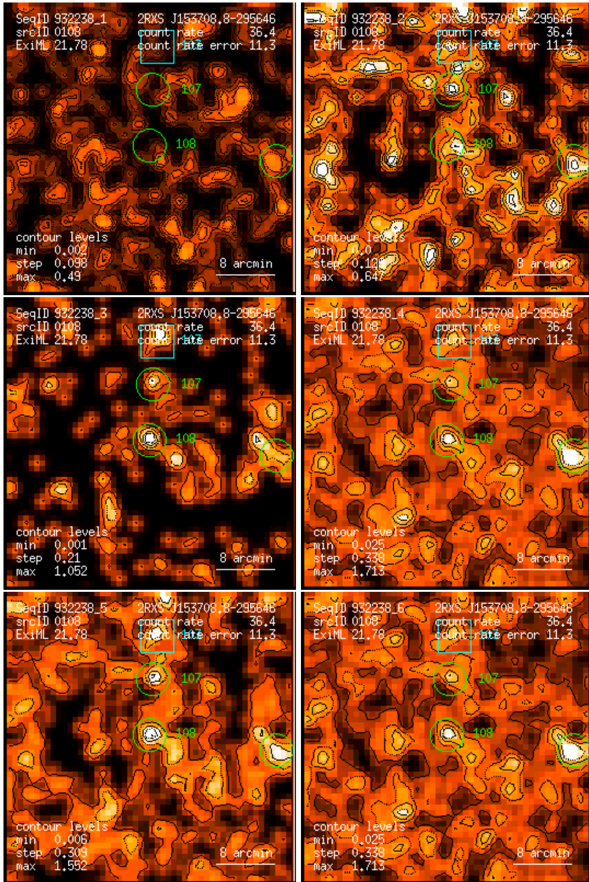
Figure 108: RASS 932238: detection 0108: band rate images, Gaussian filter: (1) PSPC channels 11 – 41, (2) 52 – 90, (3) 91 – 201, (4) 11 – 235, (5) 52 – 201, (6) 11 – 201. Broad band rates in counts/ks. Band rate contour levels in counts/ks/arcmin 2 .
