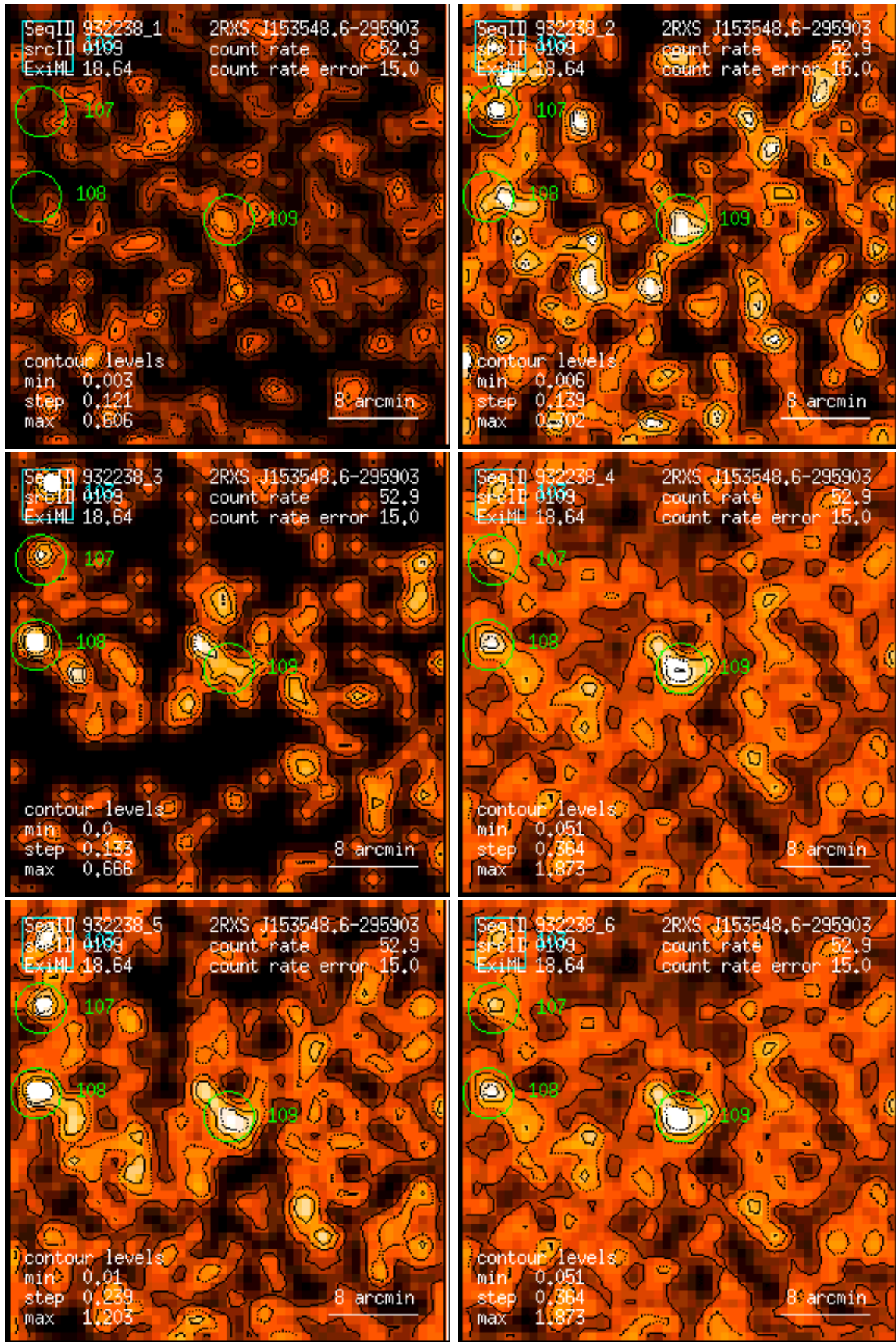
Figure 109: RASS 932238: detection 0109: band rate images, Gaussian filter: (1) PSPC channels 11 – 41, (2) 52 – 90, (3) 91 – 201, (4) 11 – 235, (5) 52 – 201, (6) 11 – 201. Broad band rates in counts/ks. Band rate contour levels in counts/ks/arcmin 2 .
