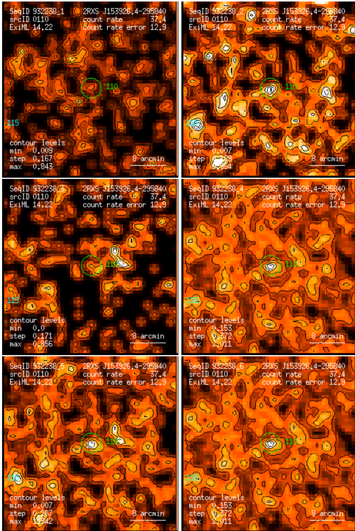
Figure 110: RASS 932238: detection 0110: band rate images, Gaussian filter: (1) PSPC channels 11 – 41, (2) 52 – 90, (3) 91 – 201, (4) 11 – 235, (5) 52 – 201, (6) 11 – 201. Broad band rates in counts/ks. Band rate contour levels in counts/ks/arcmin 2 .
