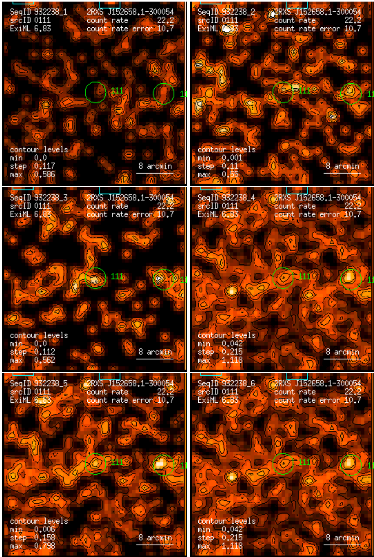
Figure 111: RASS 932238: detection 0111: band rate images, Gaussian filter: (1) PSPC channels 11 – 41, (2) 52 – 90, (3) 91 – 201, (4) 11 – 235, (5) 52 – 201, (6) 11 – 201. Broad band rates in counts/ks. Band rate contour levels in counts/ks/arcmin 2 .
