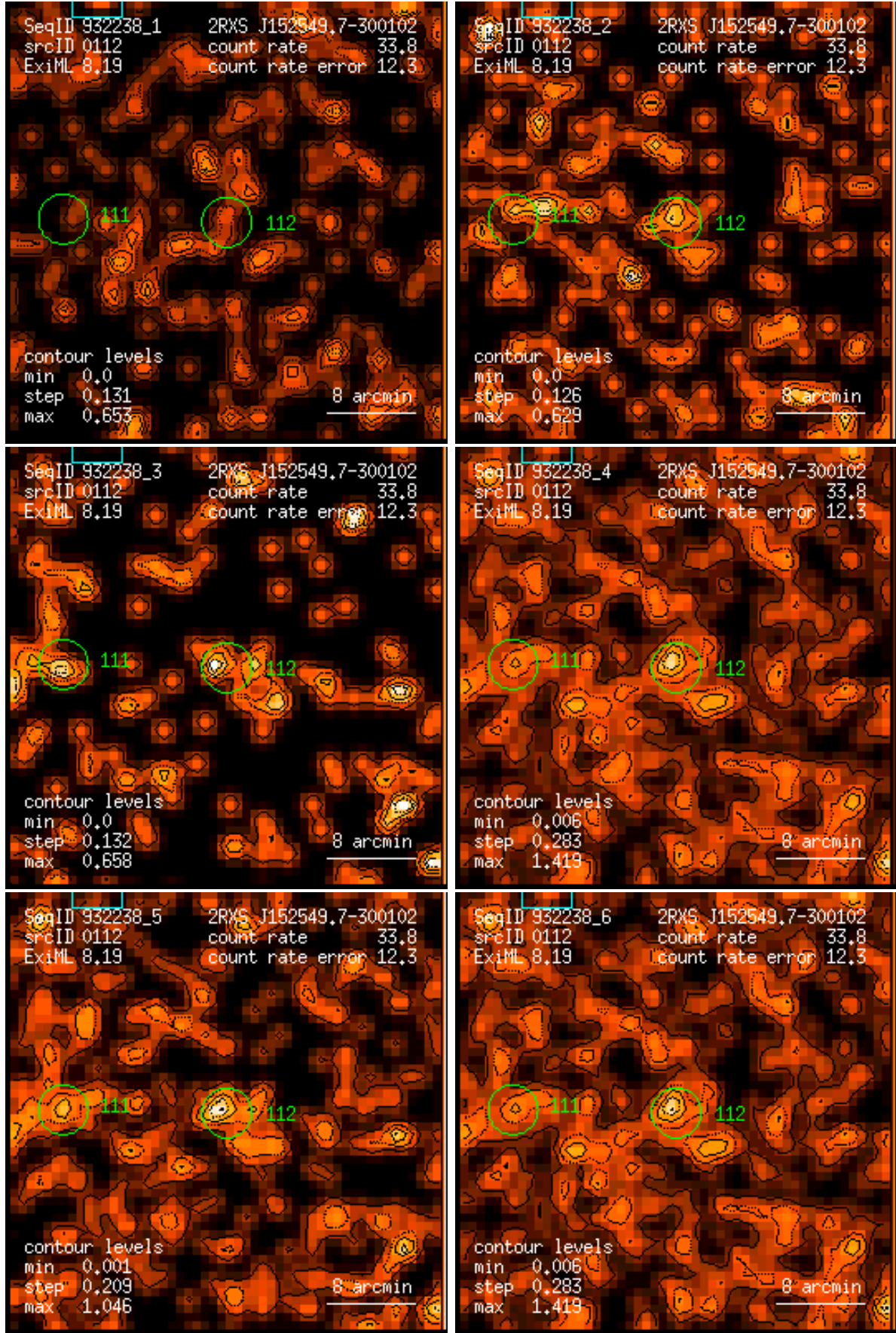
Figure 112: RASS 932238: detection 0112: band rate images, Gaussian filter: (1) PSPC channels 11 – 41, (2) 52 – 90, (3) 91 – 201, (4) 11 – 235, (5) 52 – 201, (6) 11 – 201. Broad band rates in counts/ks. Band rate contour levels in counts/ks/arcmin 2 .
