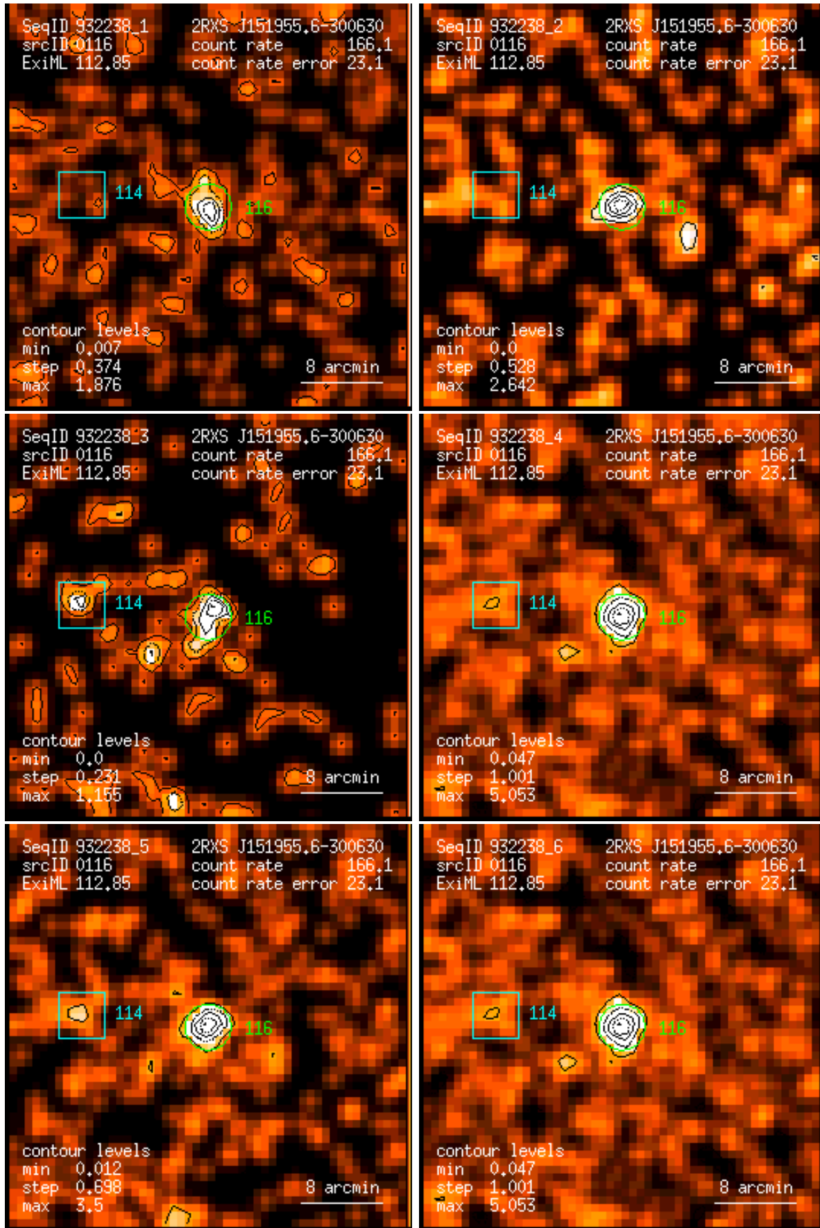
Figure 116: RASS 932238: detection 0116: band rate images, Gaussian filter: (1) PSPC channels 11 – 41, (2) 52 – 90, (3) 91 – 201, (4) 11 – 235, (5) 52 – 201, (6) 11 – 201. Broad band rates in counts/ks. Band rate contour levels in counts/ks/arcmin 2 .
