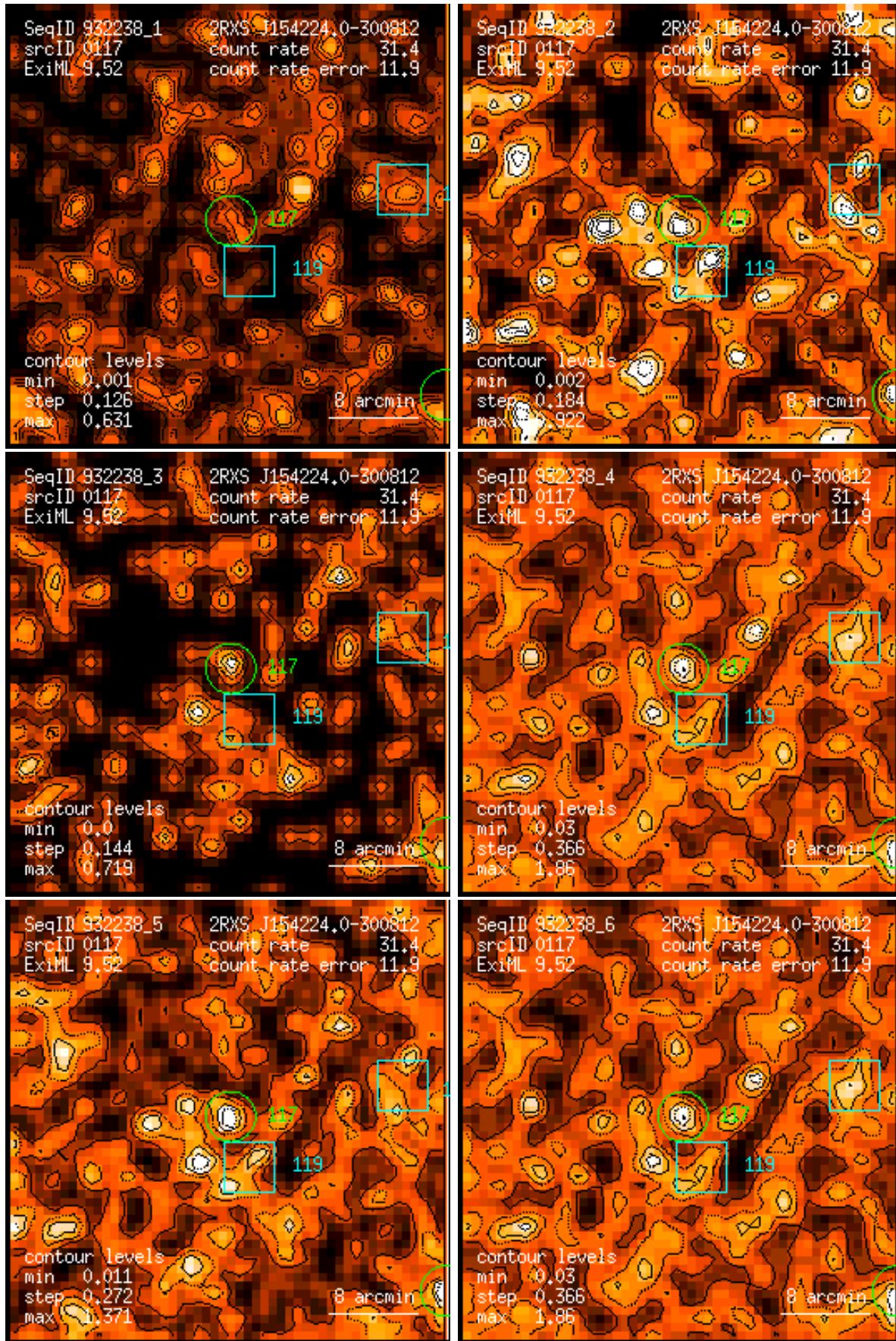
Figure 117: RASS 932238: detection 0117: band rate images, Gaussian filter: (1) PSPC channels 11 – 41, (2) 52 – 90, (3) 91 – 201, (4) 11 – 235, (5) 52 – 201, (6) 11 – 201. Broad band rates in counts/ks. Band rate contour levels in counts/ks/arcmin 2 .
