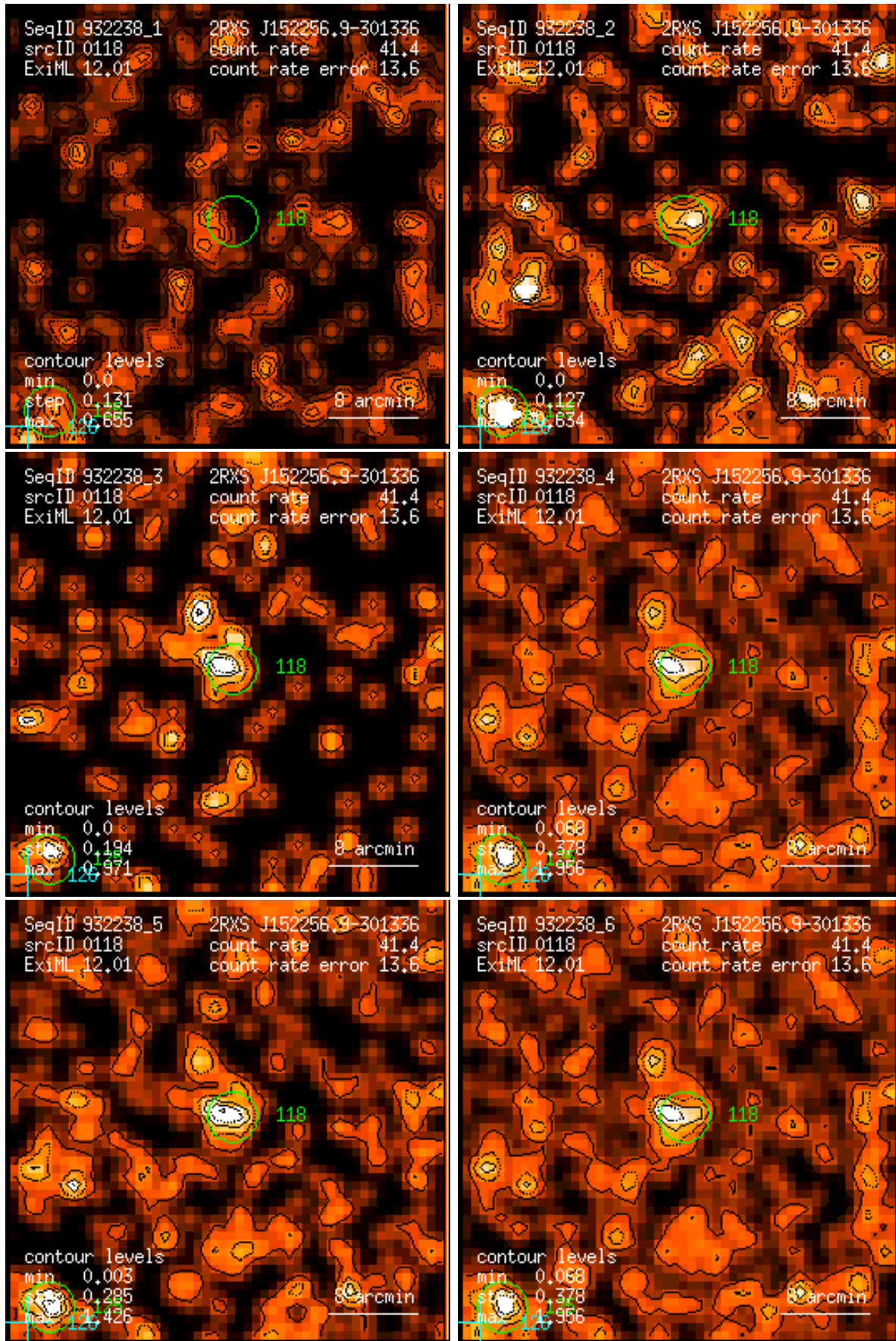
Figure 118: RASS 932238: detection 0118: band rate images, Gaussian filter: (1) PSPC channels 11 – 41, (2) 52 – 90, (3) 91 – 201, (4) 11 – 235, (5) 52 – 201, (6) 11 – 201. Broad band rates in counts/ks. Band rate contour levels in counts/ks/arcmin 2 .
