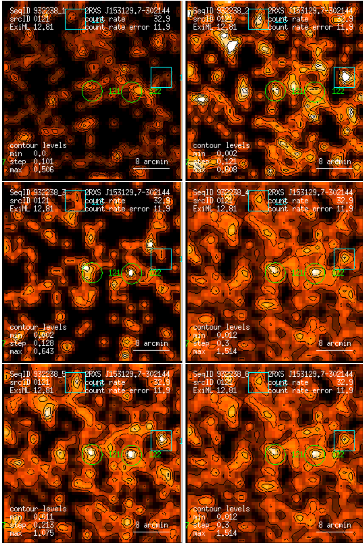
Figure 121: RASS 932238: detection 0121: band rate images, Gaussian filter: (1) PSPC channels 11 – 41, (2) 52 – 90, (3) 91 – 201, (4) 11 – 235, (5) 52 – 201, (6) 11 – 201. Broad band rates in counts/ks. Band rate contour levels in counts/ks/arcmin 2 .
