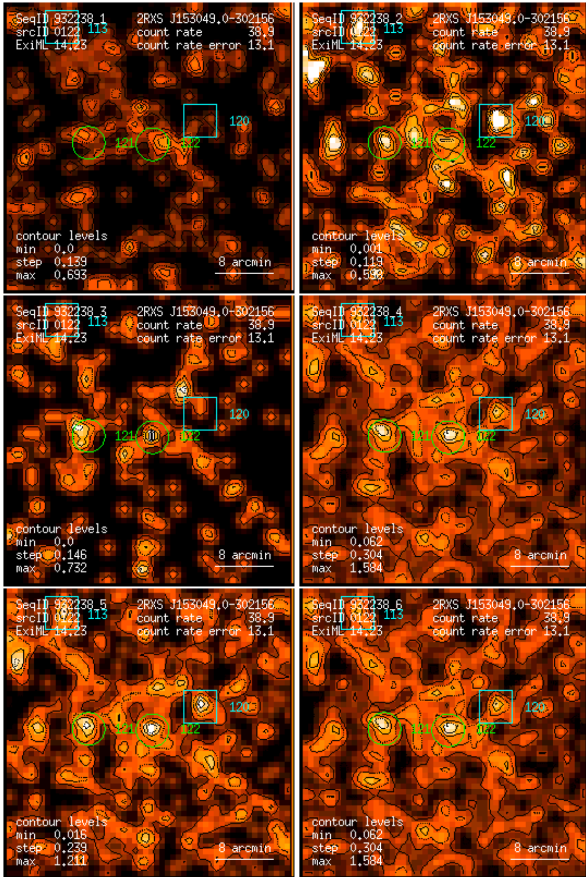
Figure 122: RASS 932238: detection 0122: band rate images, Gaussian filter: (1) PSPC channels 11 – 41, (2) 52 – 90, (3) 91 – 201, (4) 11 – 235, (5) 52 – 201, (6) 11 – 201. Broad band rates in counts/ks. Band rate contour levels in counts/ks/arcmin 2 .
