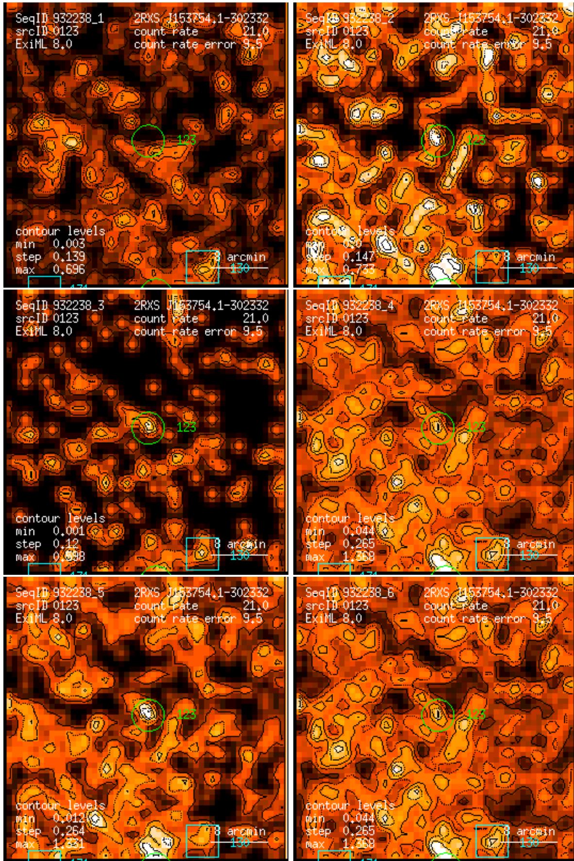
Figure 123: RASS 932238: detection 0123: band rate images, Gaussian filter: (1) PSPC channels 11 – 41, (2) 52 – 90, (3) 91 – 201, (4) 11 – 235, (5) 52 – 201, (6) 11 – 201. Broad band rates in counts/ks. Band rate contour levels in counts/ks/arcmin 2 .
