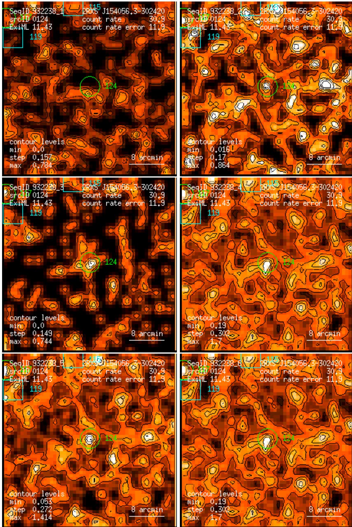
Figure 124: RASS 932238: detection 0124: band rate images, Gaussian filter: (1) PSPC channels 11 – 41, (2) 52 – 90, (3) 91 – 201, (4) 11 – 235, (5) 52 – 201, (6) 11 – 201. Broad band rates in counts/ks. Band rate contour levels in counts/ks/arcmin 2 .
