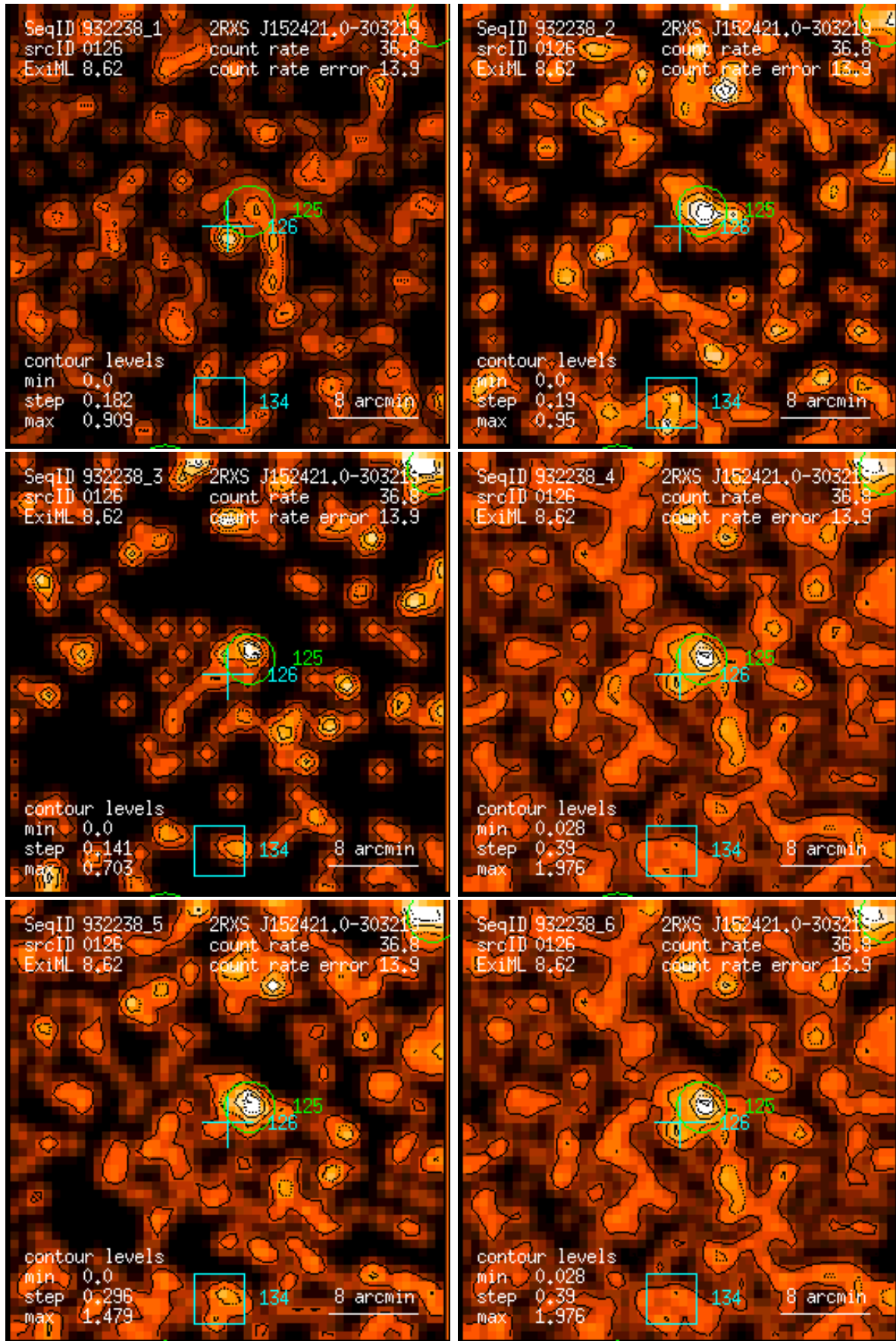
Figure 126: RASS 932238: detection 0126: band rate images, Gaussian filter: (1) PSPC channels 11 – 41, (2) 52 – 90, (3) 91 – 201, (4) 11 – 235, (5) 52 – 201, (6) 11 – 201. Broad band rates in counts/ks. Band rate contour levels in counts/ks/arcmin 2 .
