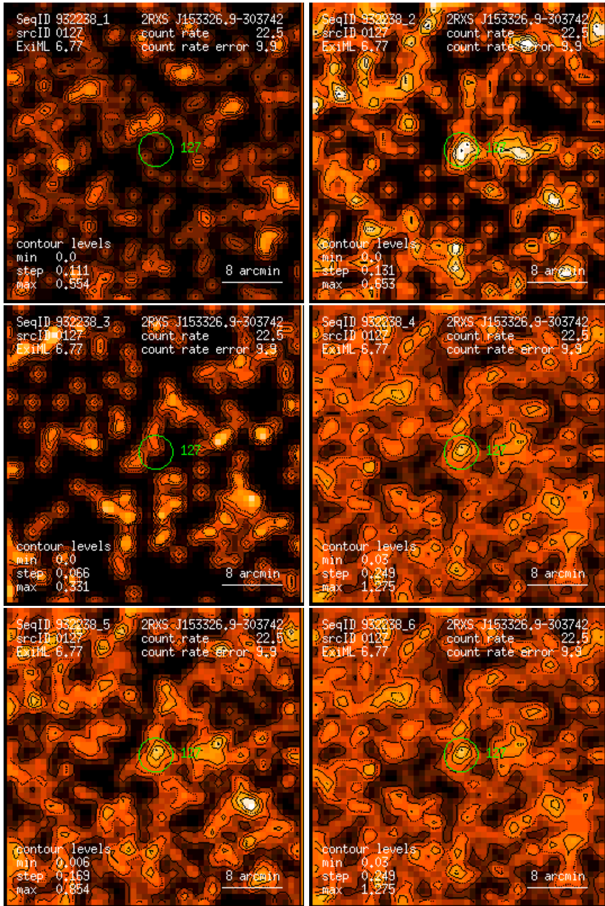
Figure 127: RASS 932238: detection 0127: band rate images, Gaussian filter: (1) PSPC channels 11 – 41, (2) 52 – 90, (3) 91 – 201, (4) 11 – 235, (5) 52 – 201, (6) 11 – 201. Broad band rates in counts/ks. Band rate contour levels in counts/ks/arcmin 2 .
