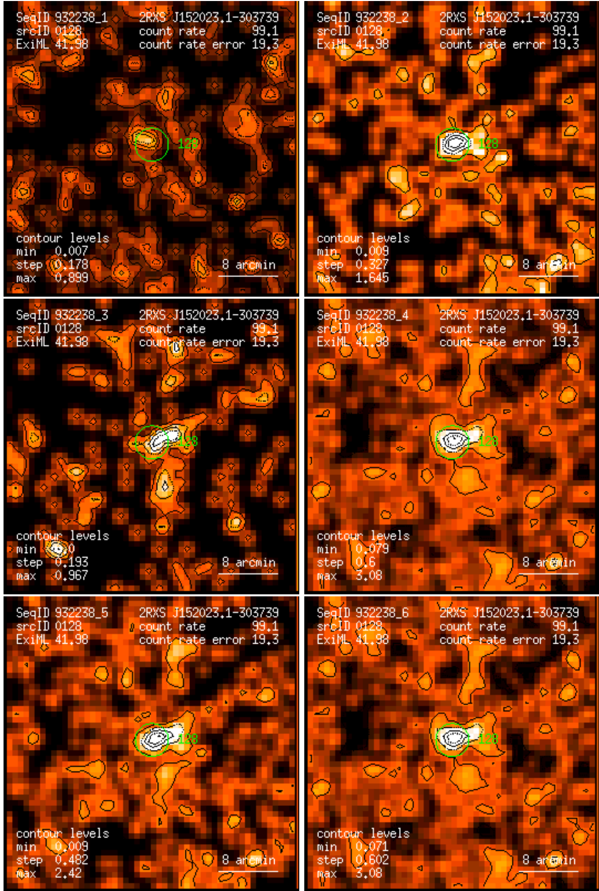
Figure 128: RASS 932238: detection 0128: band rate images, Gaussian filter: (1) PSPC channels 11 – 41, (2) 52 – 90, (3) 91 – 201, (4) 11 – 235, (5) 52 – 201, (6) 11 – 201. Broad band rates in counts/ks. Band rate contour levels in counts/ks/arcmin 2 .
