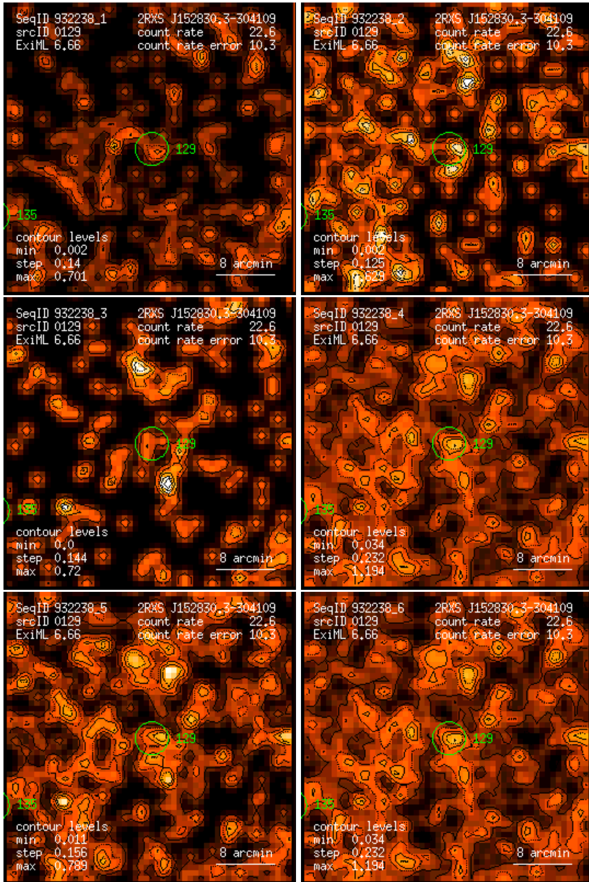
Figure 129: RASS 932238: detection 0129: band rate images, Gaussian filter: (1) PSPC channels 11 – 41, (2) 52 – 90, (3) 91 – 201, (4) 11 – 235, (5) 52 – 201, (6) 11 – 201. Broad band rates in counts/ks. Band rate contour levels in counts/ks/arcmin 2 .
