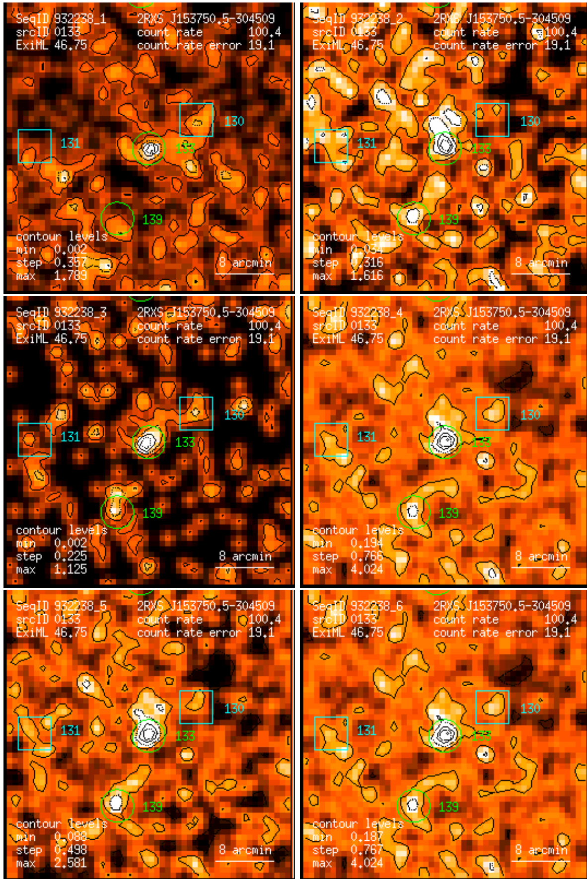
Figure 133: RASS 932238: detection 0133: band rate images, Gaussian filter: (1) PSPC channels 11 – 41, (2) 52 – 90, (3) 91 – 201, (4) 11 – 235, (5) 52 – 201, (6) 11 – 201. Broad band rates in counts/ks. Band rate contour levels in counts/ks/arcmin 2 .
