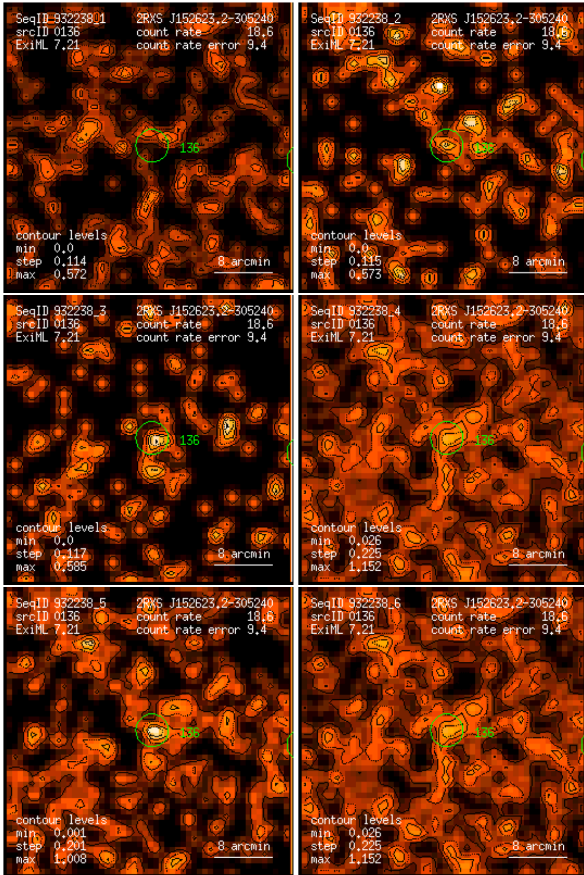
Figure 136: RASS 932238: detection 0136: band rate images, Gaussian filter: (1) PSPC channels 11 – 41, (2) 52 – 90, (3) 91 – 201, (4) 11 – 235, (5) 52 – 201, (6) 11 – 201. Broad band rates in counts/ks. Band rate contour levels in counts/ks/arcmin 2 .
