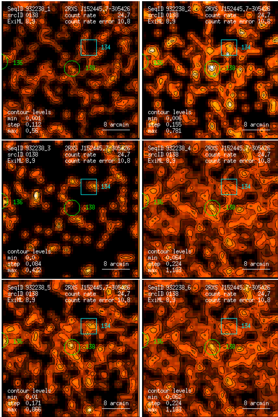
Figure 138: RASS 932238: detection 0138: band rate images, Gaussian filter: (1) PSPC channels 11 – 41, (2) 52 – 90, (3) 91 – 201, (4) 11 – 235, (5) 52 – 201, (6) 11 – 201. Broad band rates in counts/ks. Band rate contour levels in counts/ks/arcmin 2 .
