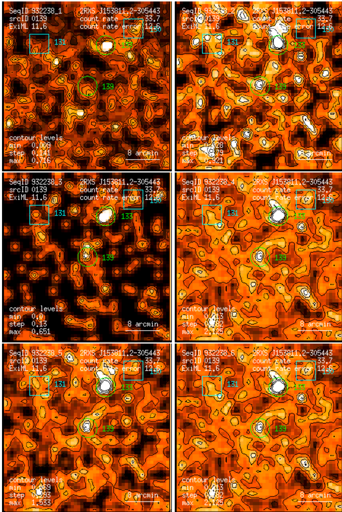
Figure 139: RASS 932238: detection 0139: band rate images, Gaussian filter: (1) PSPC channels 11 – 41, (2) 52 – 90, (3) 91 – 201, (4) 11 – 235, (5) 52 – 201, (6) 11 – 201. Broad band rates in counts/ks. Band rate contour levels in counts/ks/arcmin 2 .
