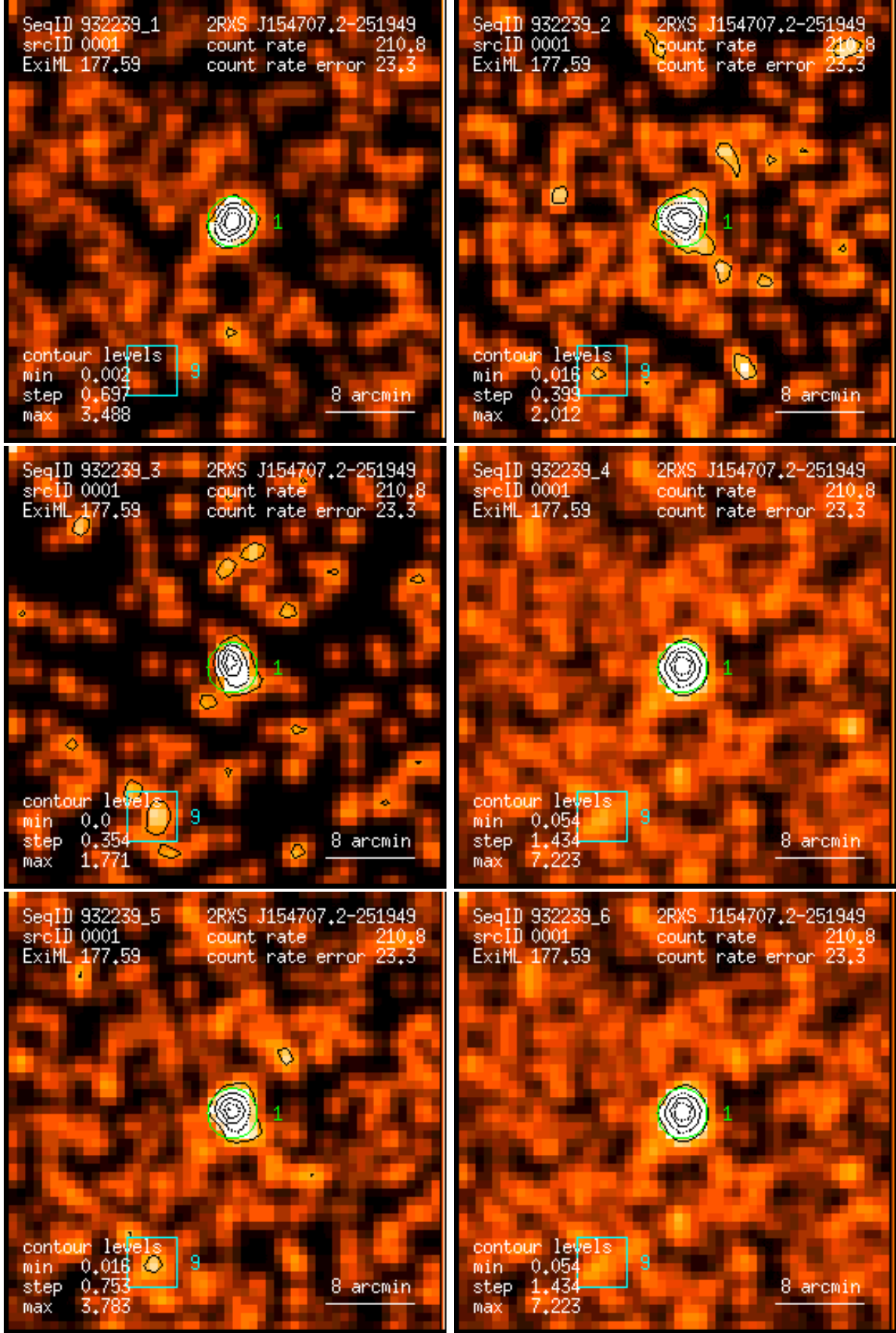
Figure 1: RASS 932239: detection 0001: band rate images, Gaussian filter: (1) PSPC channels 11 – 41, (2) 52 – 90, (3) 91 – 201, (4) 11 – 235, (5) 52 – 201, (6) 11 – 201. Broad band rates in counts/ks. Band rate contour levels in counts/ks/arcmin 2 .
