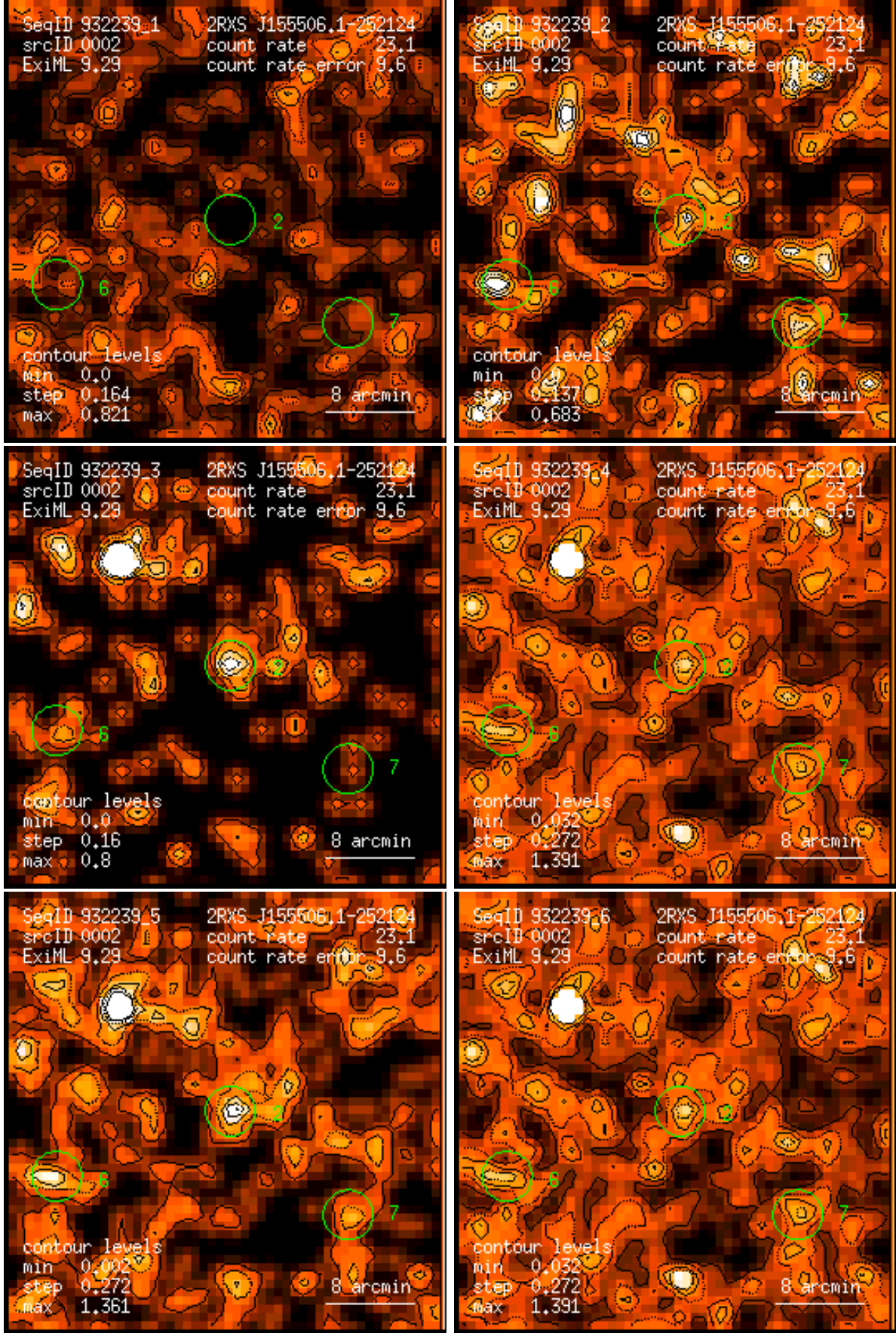
Figure 2: RASS 932239: detection 0002: band rate images, Gaussian filter: (1) PSPC channels 11 – 41, (2) 52 – 90, (3) 91 – 201, (4) 11 – 235, (5) 52 – 201, (6) 11 – 201. Broad band rates in counts/ks. Band rate contour levels in counts/ks/arcmin 2 .
